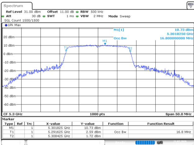
802.11a_5300MHz_Chain 4
