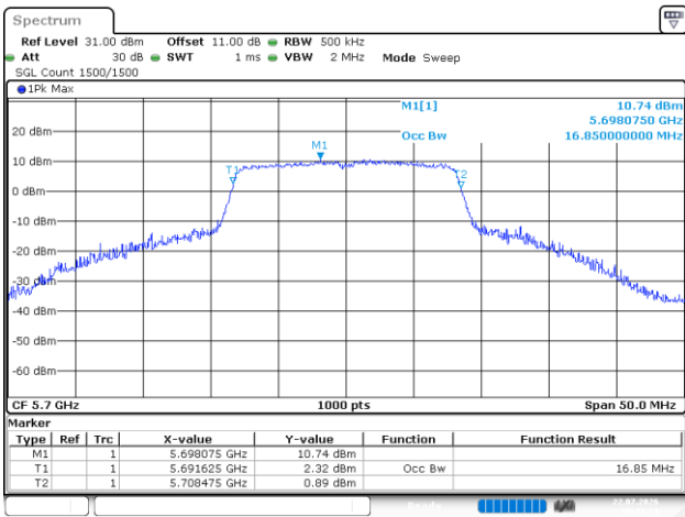
802.11a_5700MHz_Chain 4
