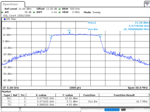
802.11a_5580MHz_Chain 0
