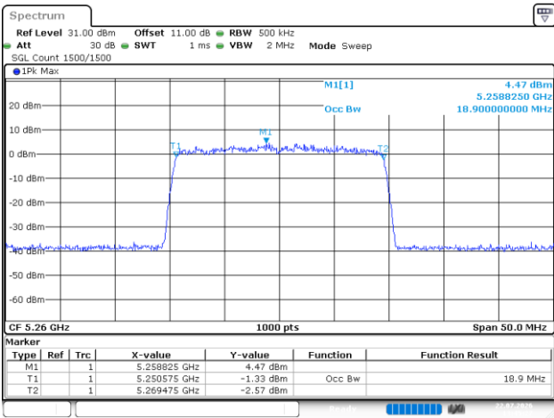
802.11be20_5260MHz_RU_Full_Chain 3
