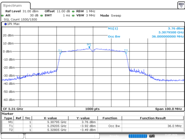
802.11ac40_5310MHz_Chain 3
