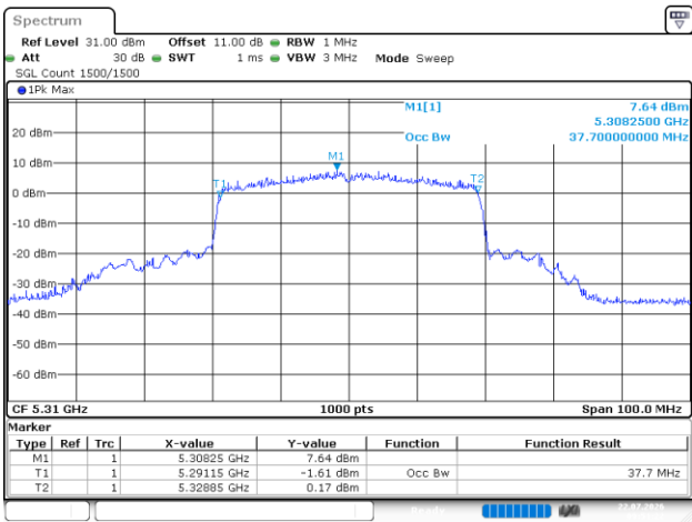
802.11be40_5310MHz_RU_Full_Chain 3
