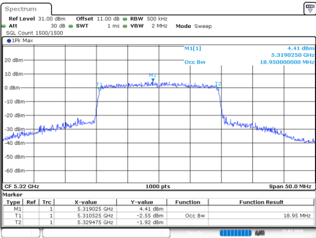
802.11be20_5320MHz_RU_Full_Chain 0
