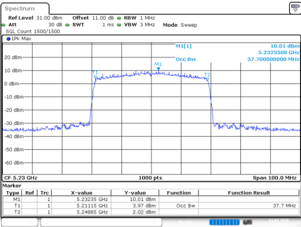
802.11be40_5230MHz_RU_Full_Chain 3
