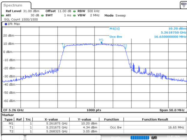
802.11a_5260MHz_Chain 3
