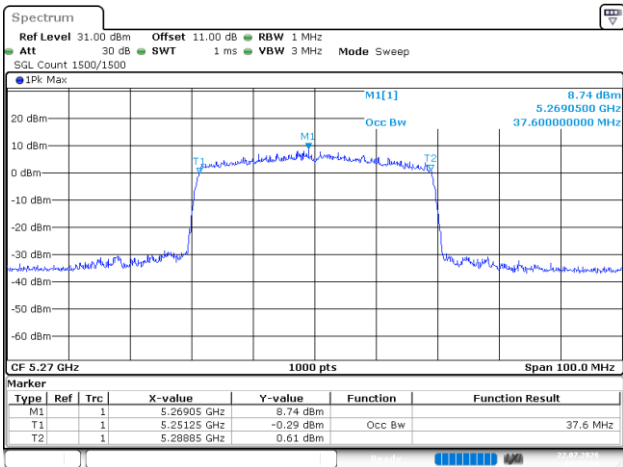
802.11be40_5270MHz_RU_Full_Chain 0
