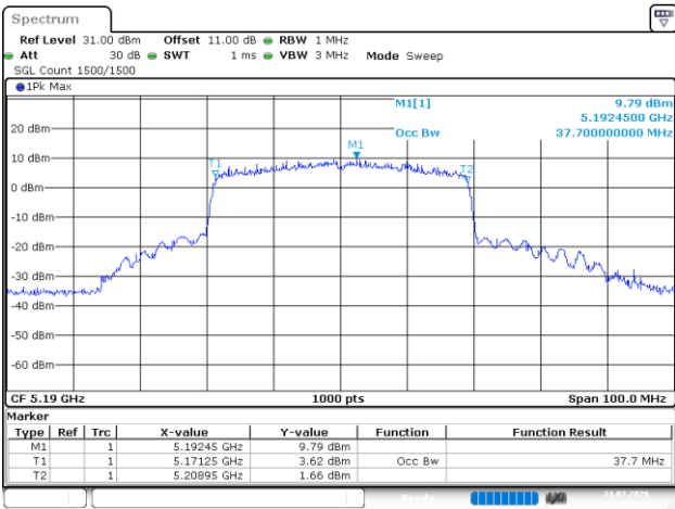
802.11be40_5190MHz_RU_Full_Chain 4
