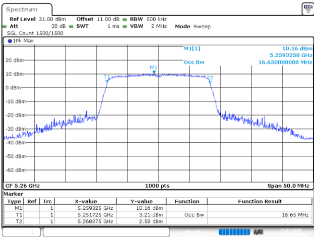
802.11a_5260MHz_Chain 2
