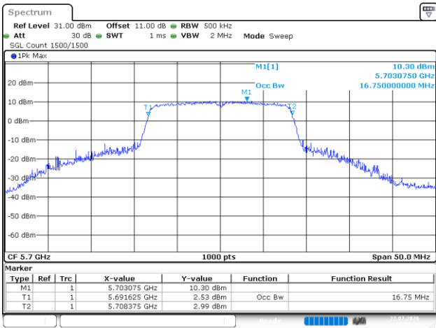
802.11a_5700MHz_Chain 0
