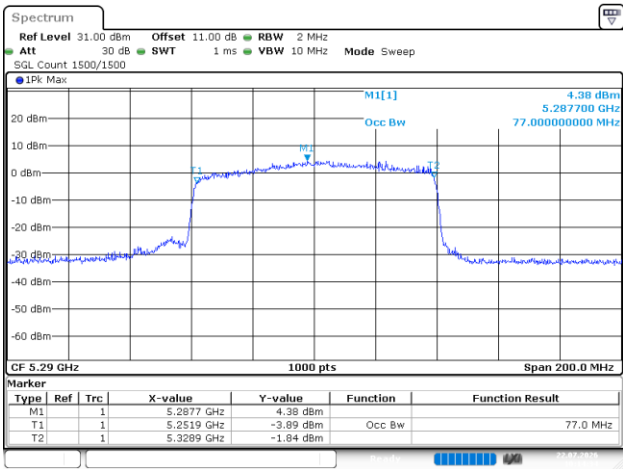
802.11be80_5290MHz_RU_Full_Chain 1
