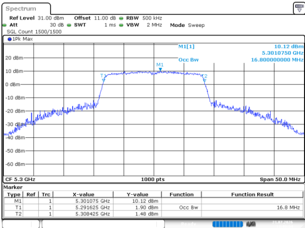
802.11a_5300MHz_Chain 3
