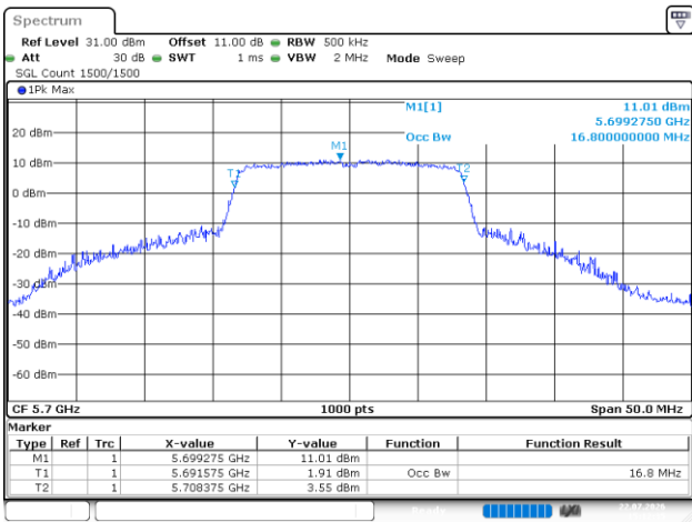
802.11a_5700MHz_Chain 1
