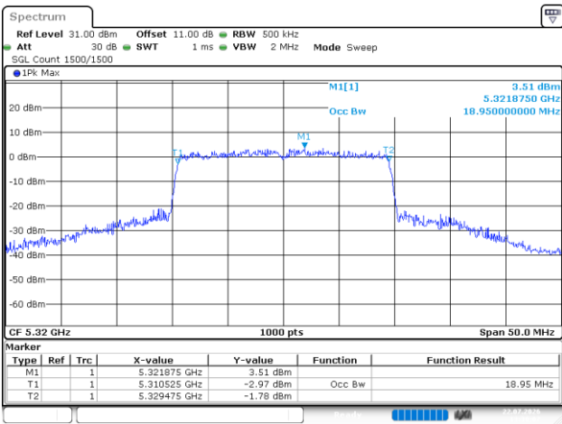
802.11be20_5320MHz_RU_Full_Chain 1
