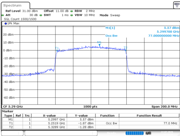
802.11be80_5290MHz_RU_Full_Chain 4
