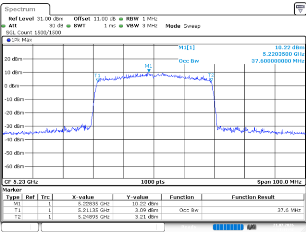
802.11be40_5230MHz_RU_Full_Chain 4
