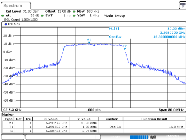
802.11a_5300MHz_Chain 2
