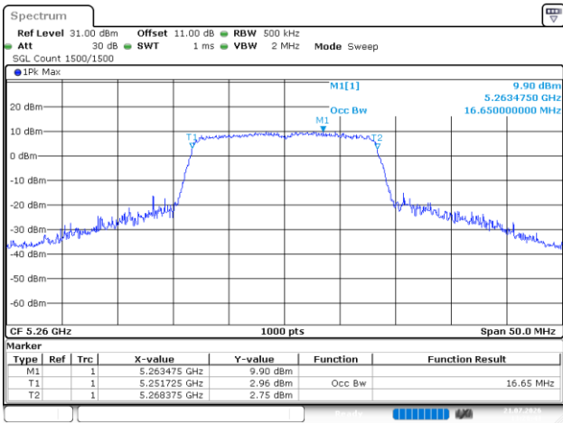
802.11a_5260MHz_Chain 1
