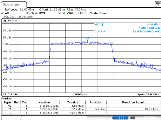
802.11be20_5300MHz_RU_Full_Chain 4
