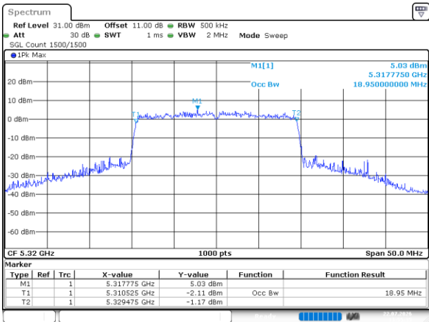
802.11be20_5320MHz_RU_Full_Chain 4
