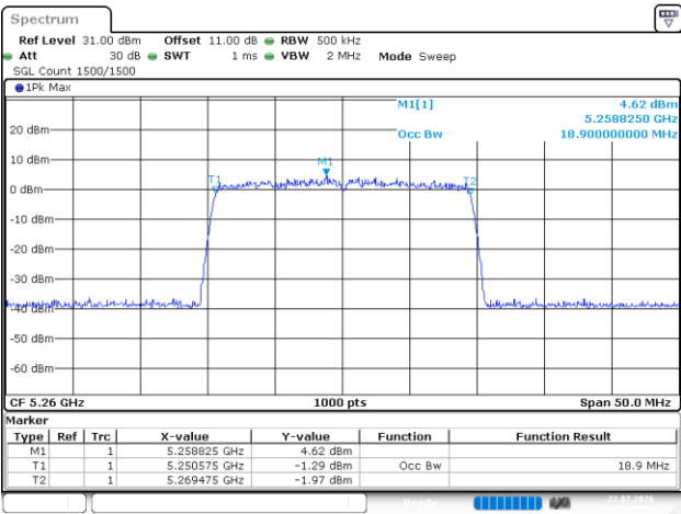
802.11be20_5260MHz_RU_Full_Chain 0
