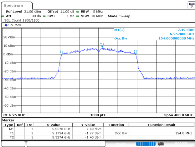
802.11ac160_5250MHz_Chain 0
