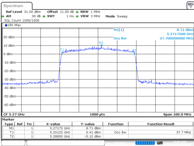
802.11be40_5270MHz_RU_Full_Chain 4
