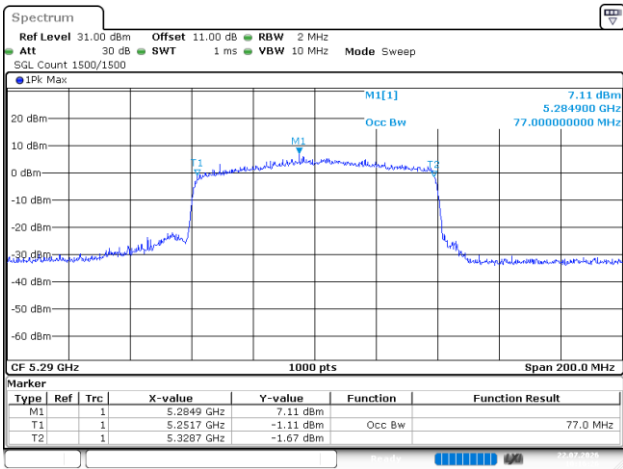
802.11be80_5290MHz_RU_Full_Chain 2
