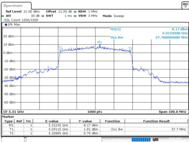
802.11be40_5310MHz_RU_Full_Chain 0
