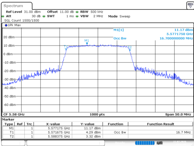
802.11a_5580MHz_Chain 1
