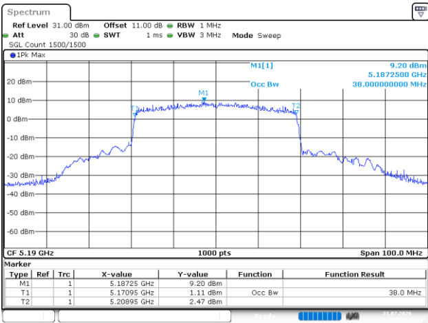
802.11be40_5190MHz_RU_Full_Chain 3
