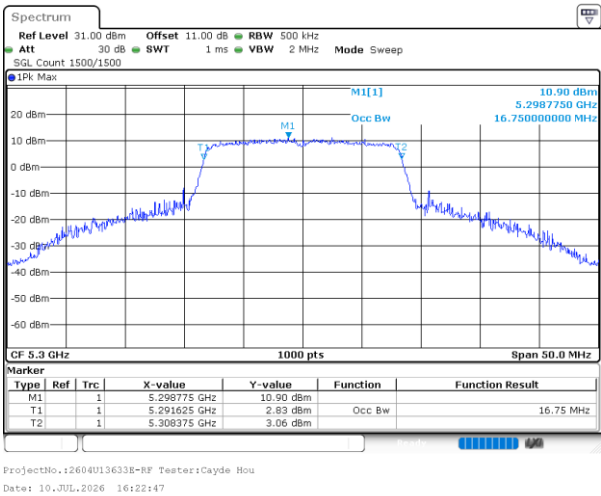
802.11a_5300MHz_Chain 0
