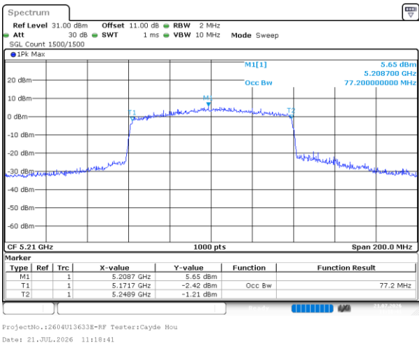
802.11be80_5210MHz_RU_Full_Chain 3
