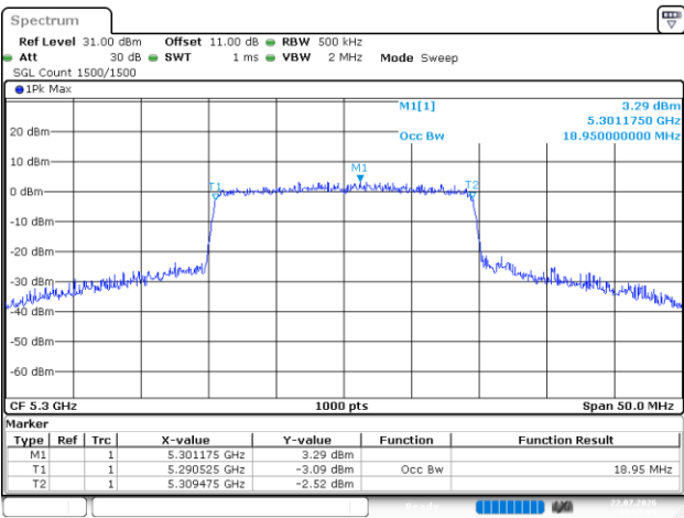
802.11be20_5300MHz_RU_Full_Chain 1
