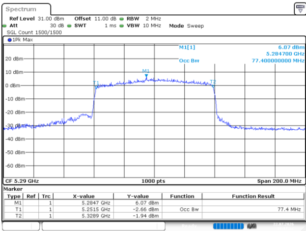
802.11be80_5290MHz_RU_Full_Chain 3
