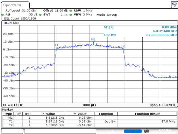
802.11be40_5310MHz_RU_Full_Chain 2
