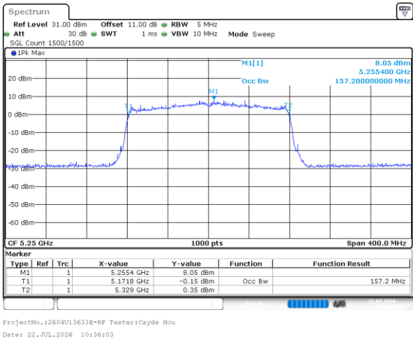
802.11be160_5250MHz_RU_Full_Chain 4
