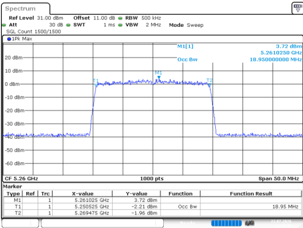
802.11be20_5260MHz_RU_Full_Chain 1
