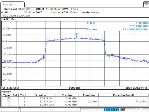
802.11be80_5210MHz_RU_Full_Chain 0
