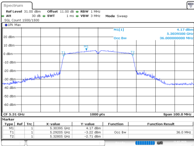
802.11ac40_5310MHz_Chain 4
