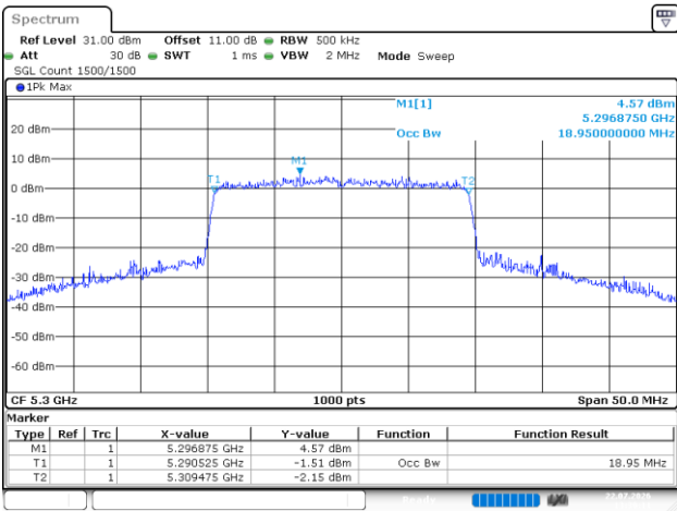
802.11be20_5300MHz_RU_Full_Chain 0
