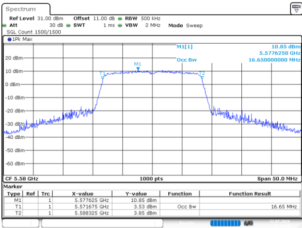
802.11a_5580MHz_Chain 4
