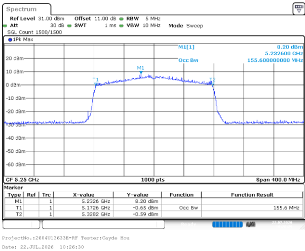
802.11be160_5250MHz_RU_Full_Chain 2
