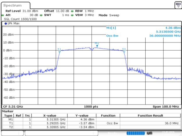
802.11ac40_5310MHz_Chain 0
