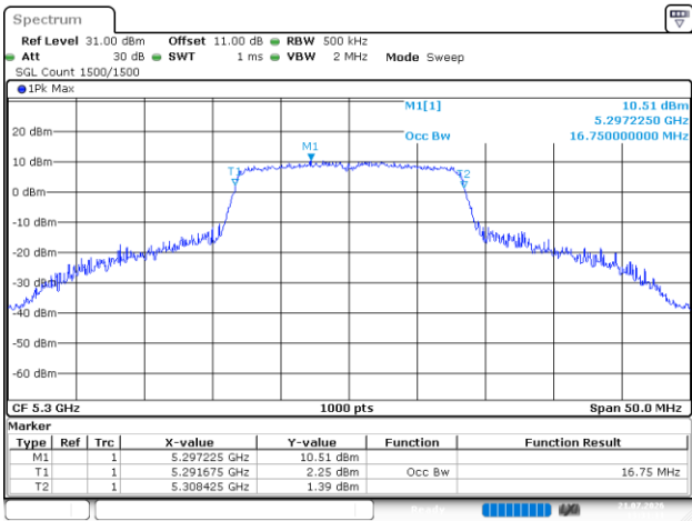
802.11a_5300MHz_Chain 1
