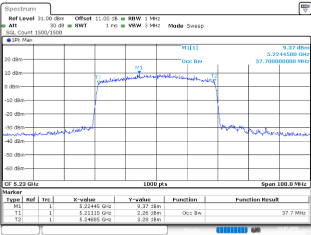
802.11be40_5230MHz_RU_Full_Chain 2
