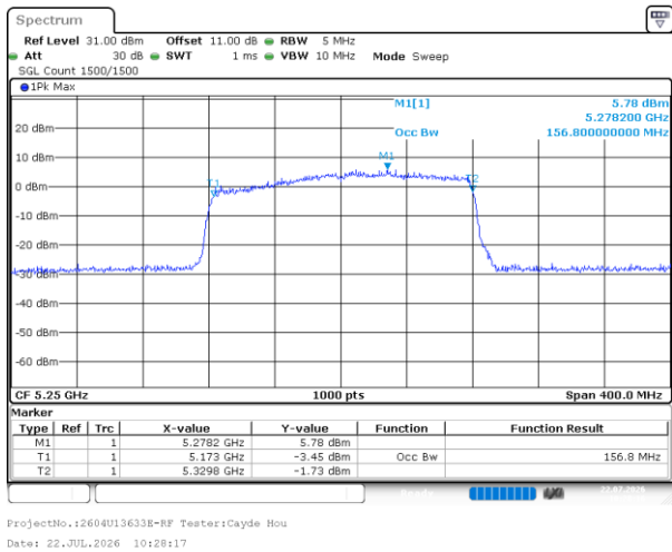
802.11be160_5250MHz_RU_Full_Chain 3
