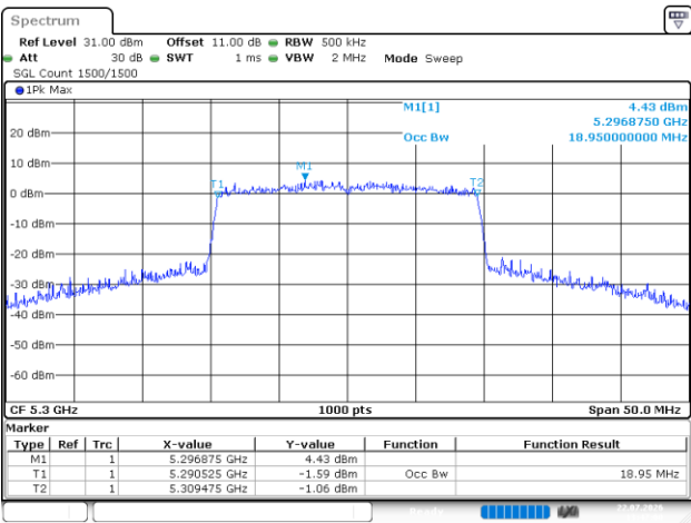
802.11be20_5300MHz_RU_Full_Chain 3
