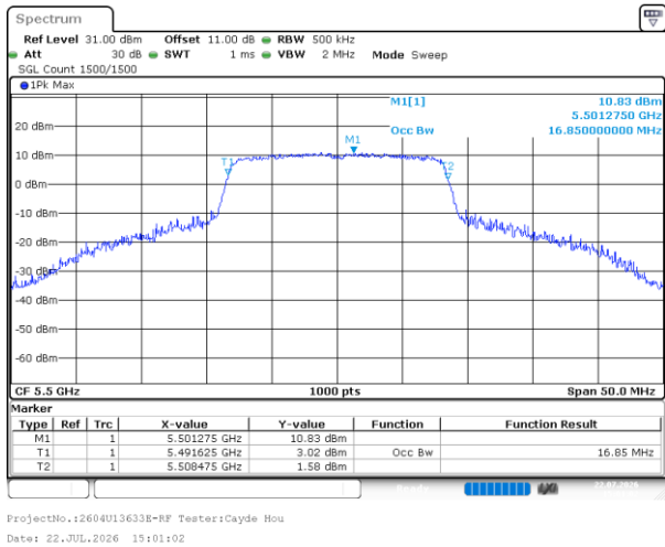
802.11a_5500MHz_Chain 0
