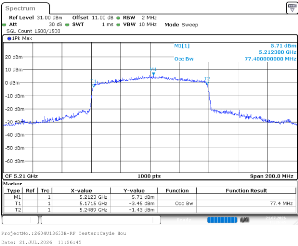
802.11be80_5210MHz_RU_Full_Chain 4
