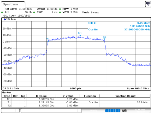
802.11be40_5310MHz_RU_Full_Chain 4
