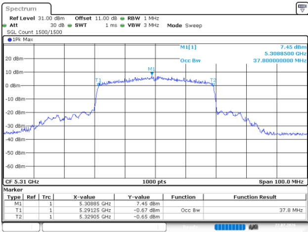
802.11be40_5310MHz_RU_Full_Chain 1
