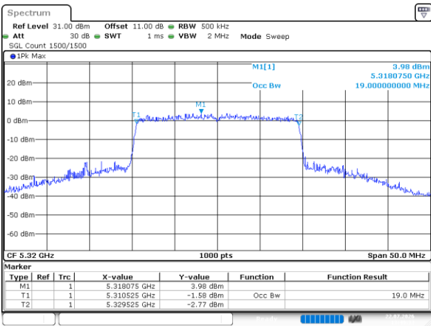
802.11be20_5320MHz_RU_Full_Chain 3
