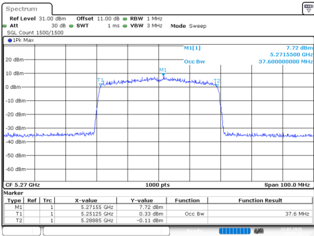
802.11be40_5270MHz_RU_Full_Chain 3
