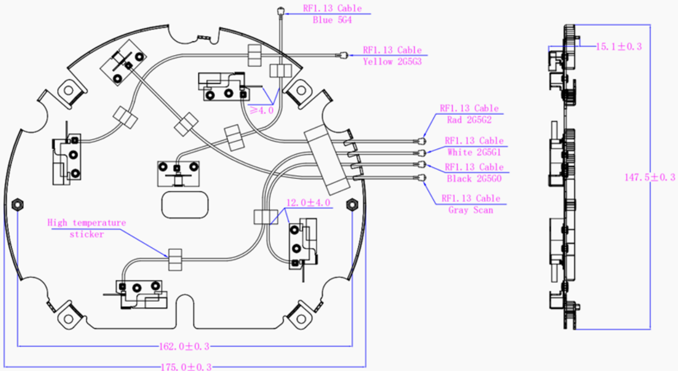
总成图 Mechanical Drawing(unit:mm)
