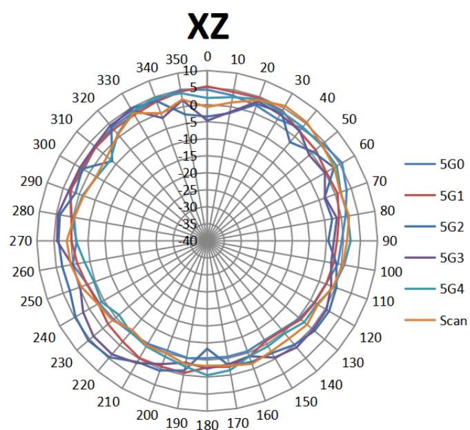
5G Antenna Radiation Patterns(unit:dBi)
