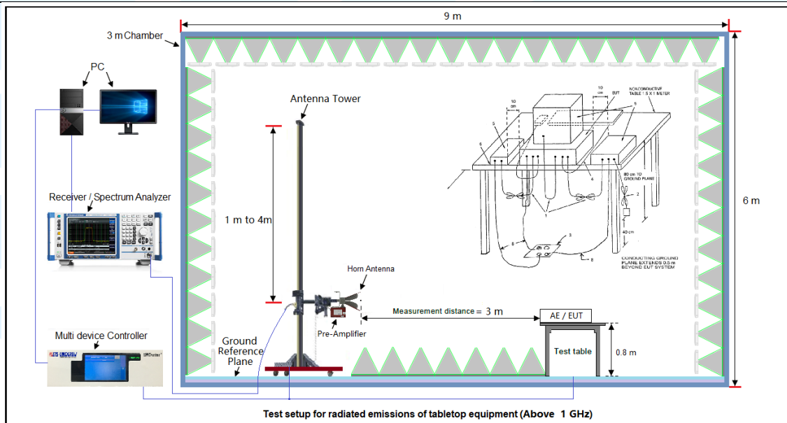
Figure 2. Above 1GHz
