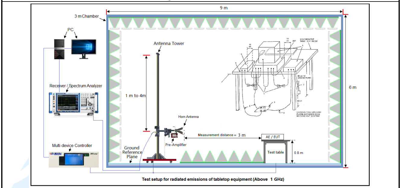
Figure 2. Above 1GHz
