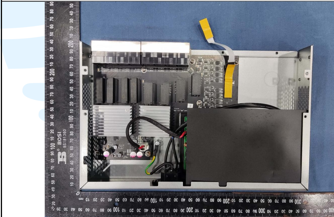
EUT Photo _ Configuring the Build-in Power 2
