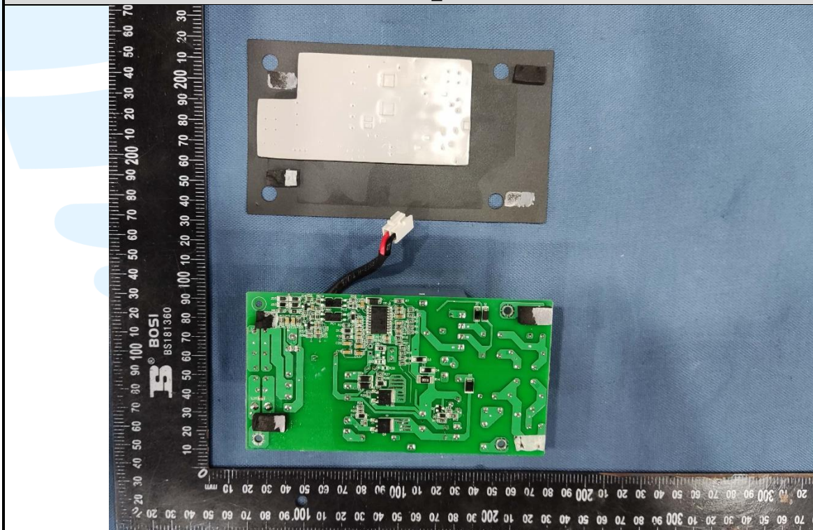
EUT Photo _ Build-in Power 2
