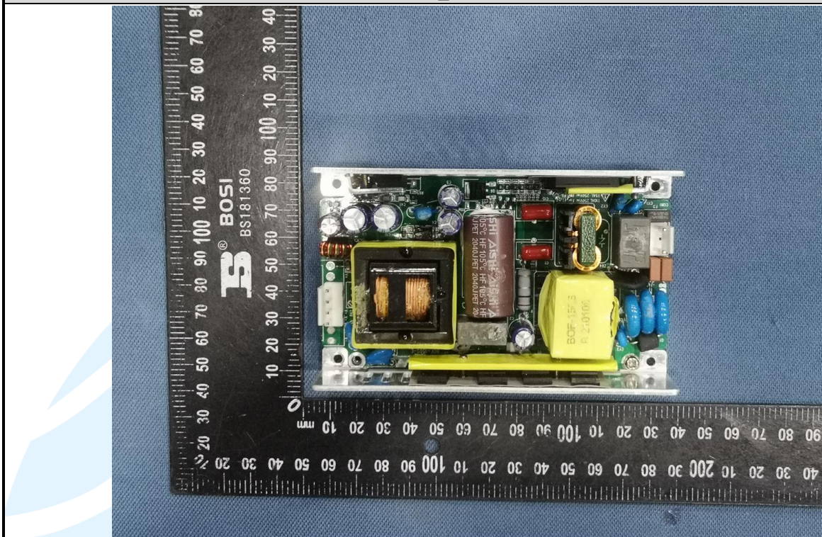
EUT Photo _ Build-in Power 1
