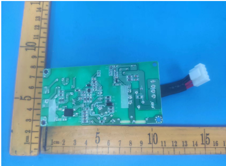
Main board
