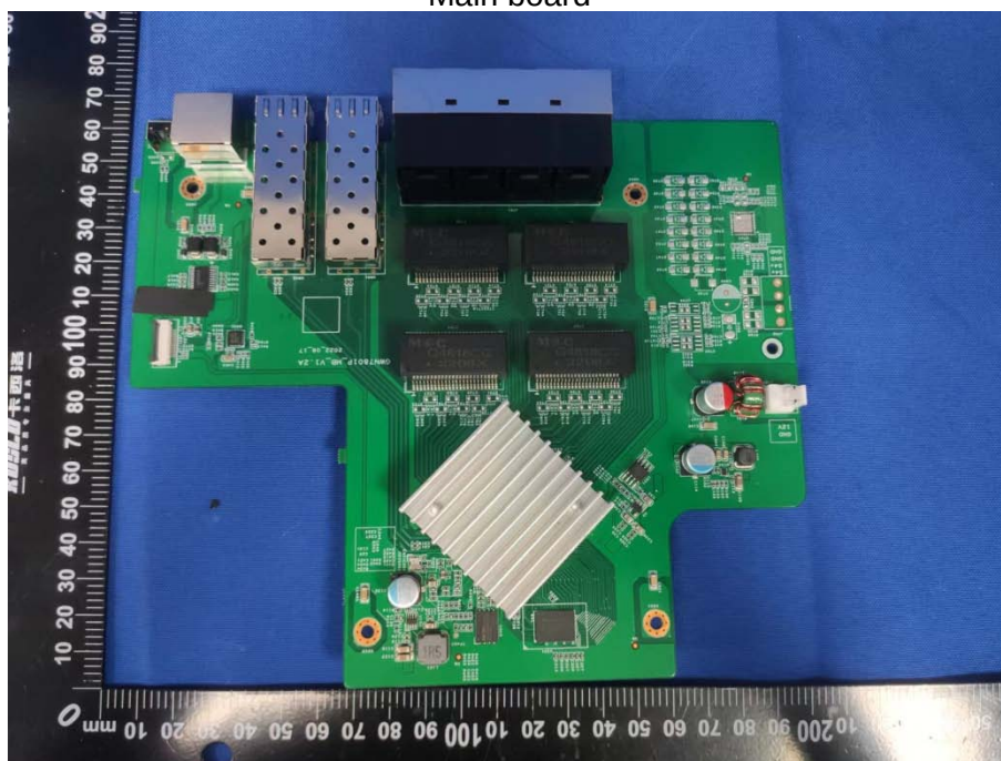
Main board
