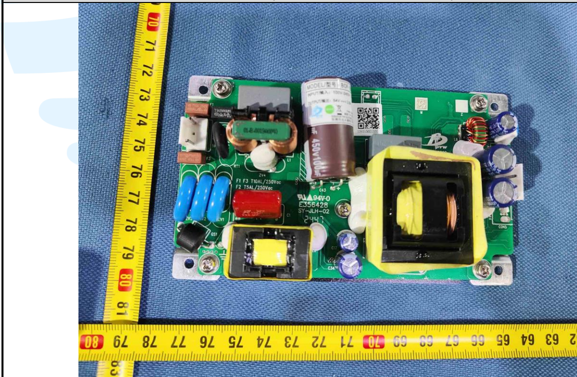
EUT Photo(Power board: BOF-150S54E)
