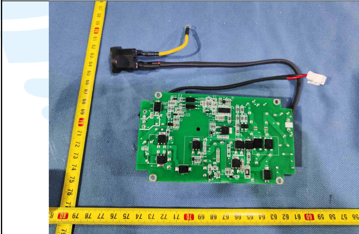
EUT Photo(Power board: UES150-540280SPA3-OP)
