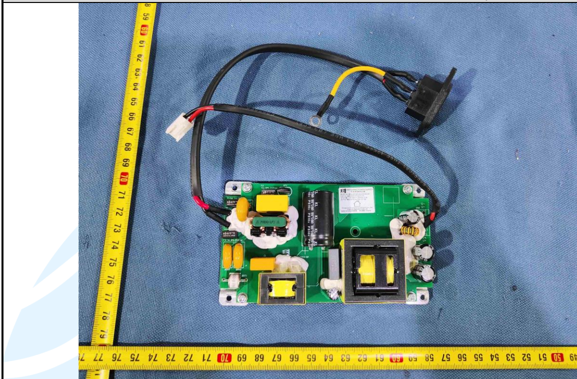
EUT Photo(Power board: UES150-540280SPA3-OP)
