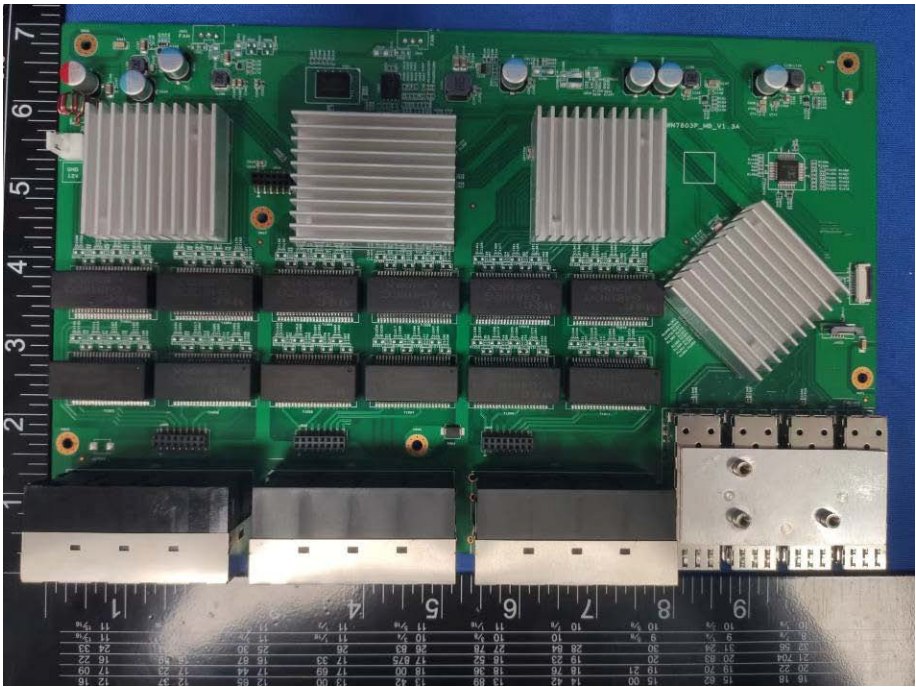
Main Board
