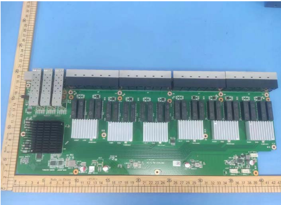
Main board
