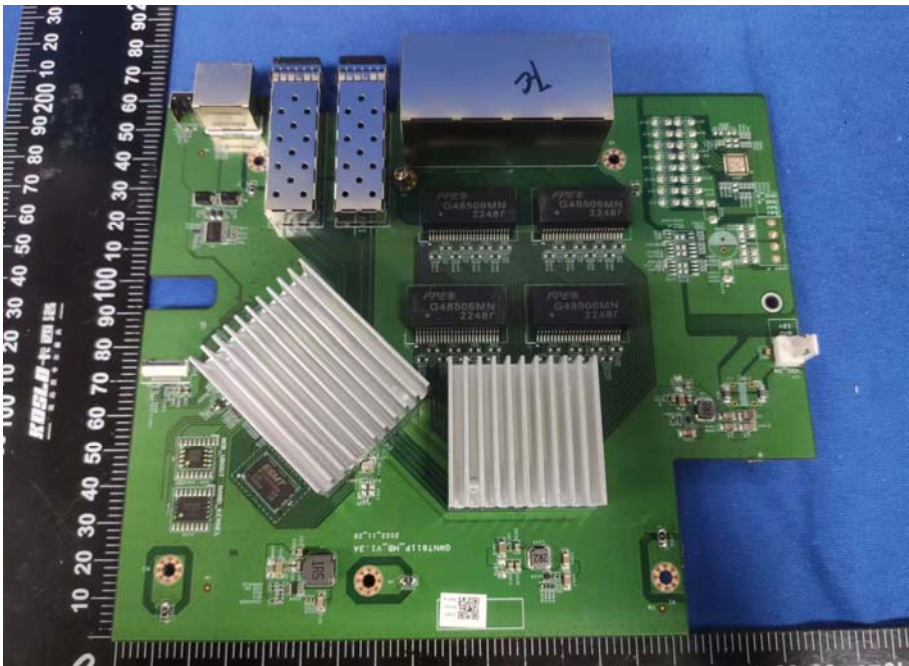
Main board
