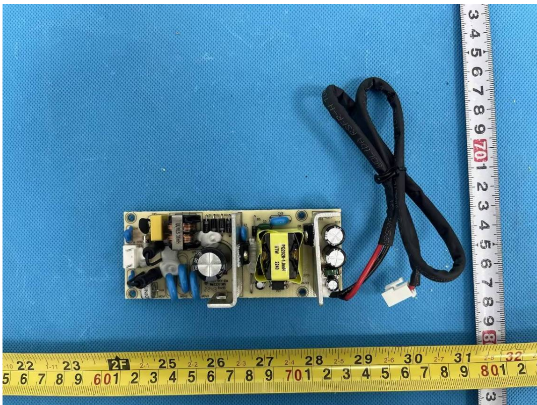
Power #1: R0001B(RB030W05-1302300)
