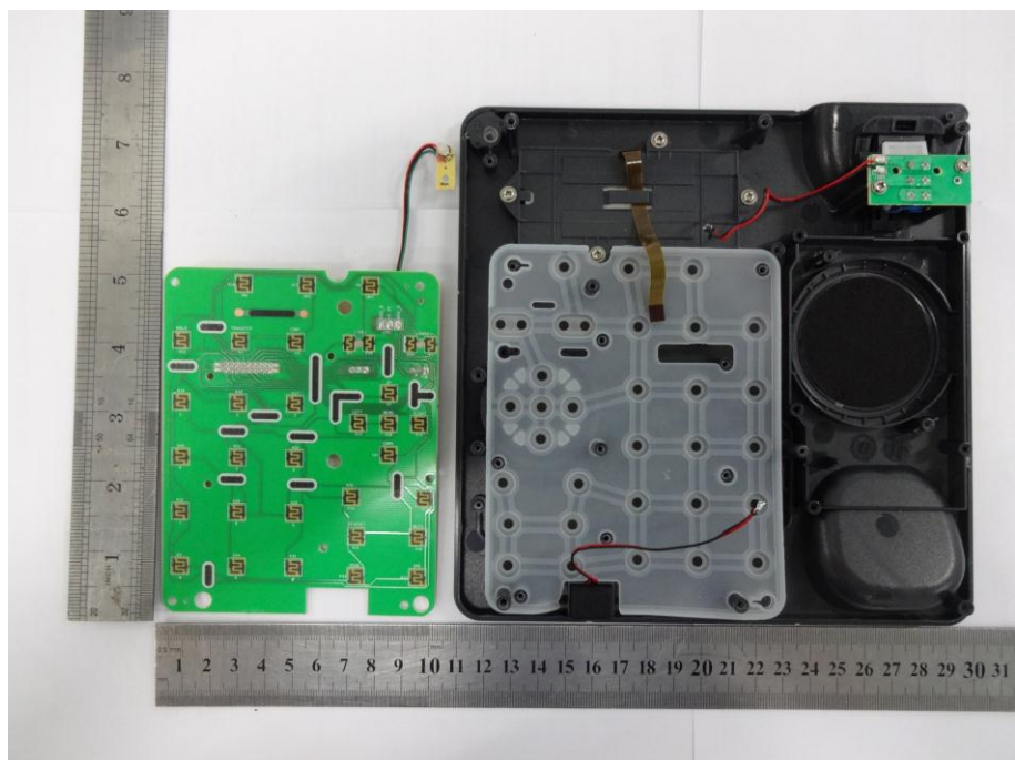
EUT-Uncovered View #4
