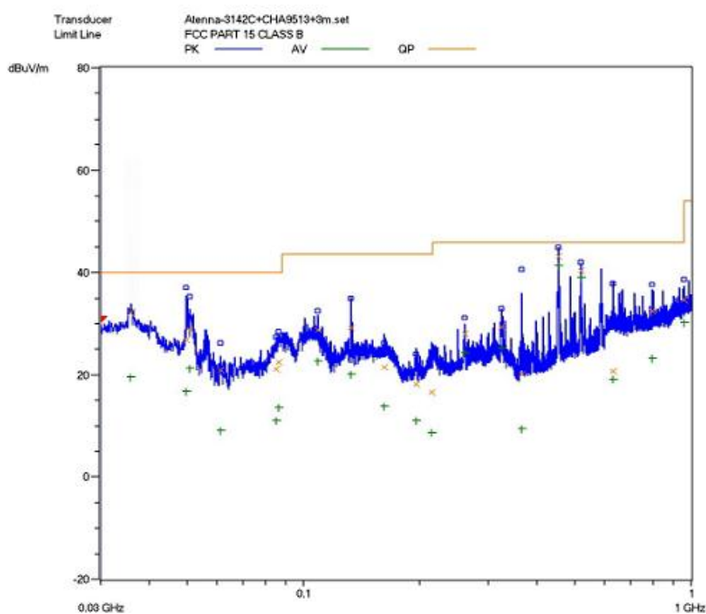
Vertical:Radiated Emission Test Plot
