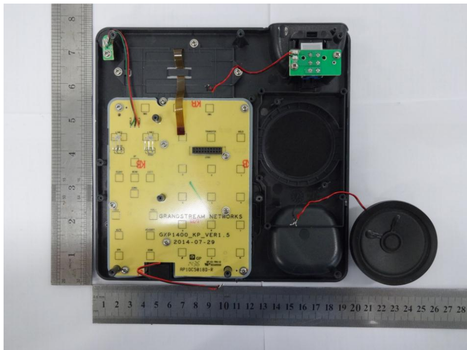
EUT-Uncovered View #3
