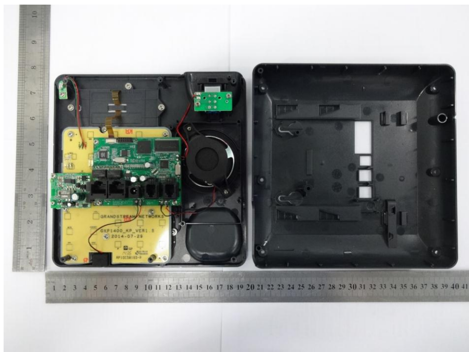
EUT-Uncovered View #1
