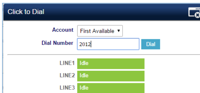
Figure 4: Click-to-Dial
