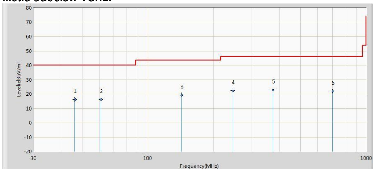
Horizontal:Radiated Emission Test Plot
