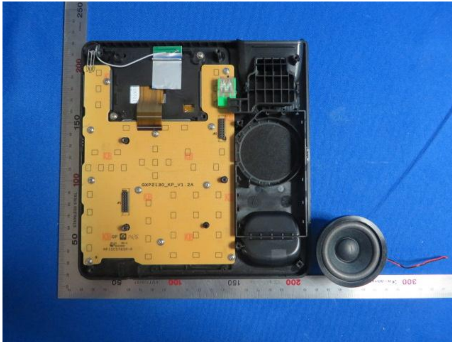
EUT-Uncovered View #3
