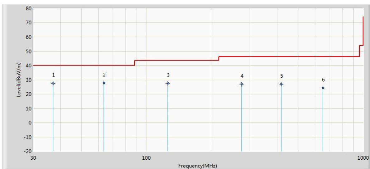
Vertical:Radiated Emission Test Plot
