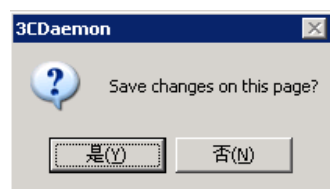
Figure 164 Confirm Changes
