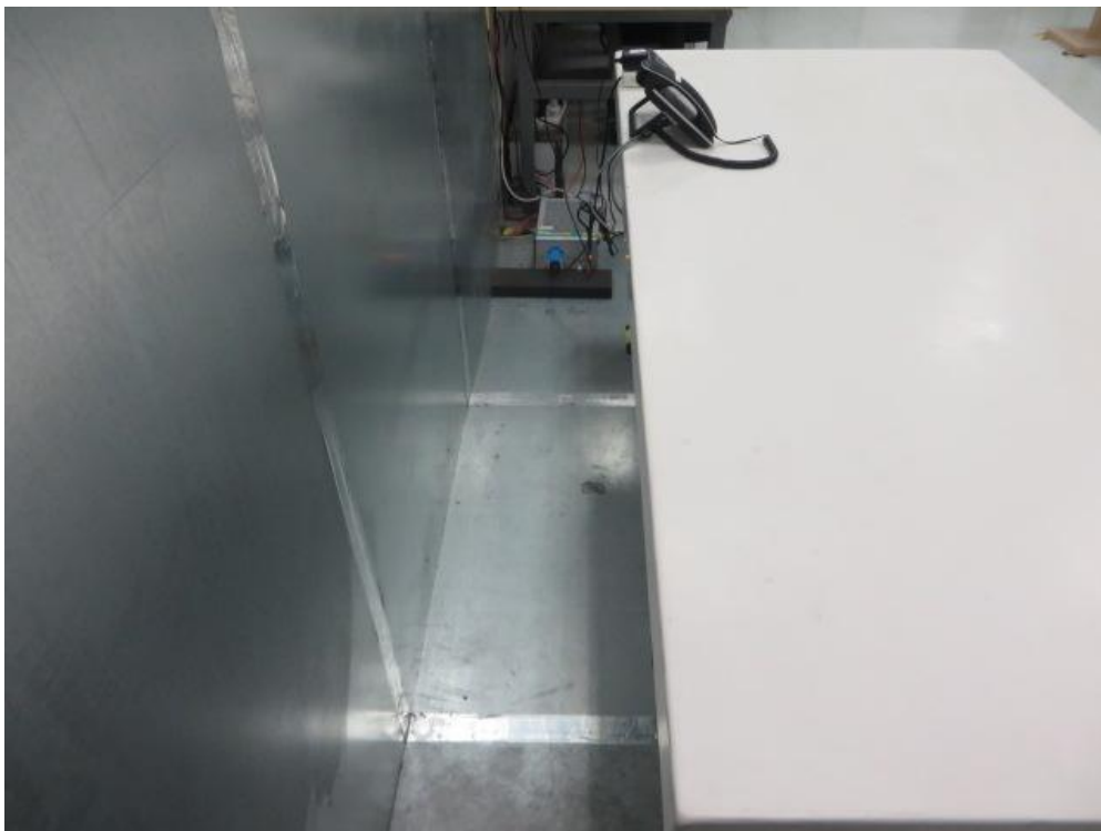
Description: Back view of Conducted Emission Test Setup (Adapter #2)
