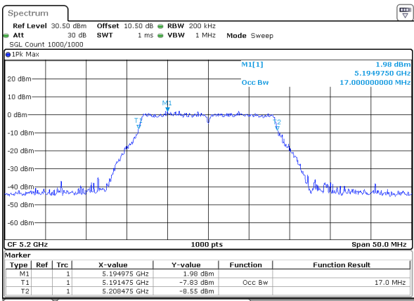
802.11a_5200MHz
