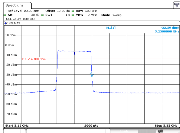
802.11ax40_5230MHz_RU_Full
