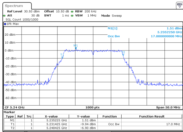
802.11a_5240MHz
