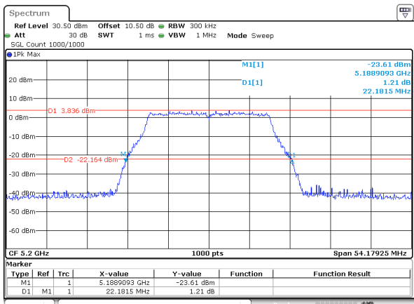
802.11a_5200MHz
