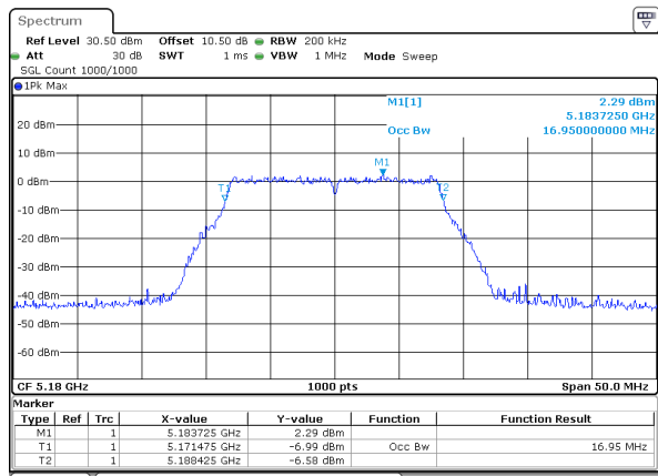
802.11a_5180MHz
