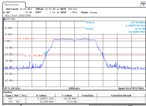
802.11a_5180MHz
