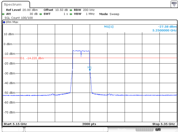
802.11ax20_5240MHz_RU_Full
