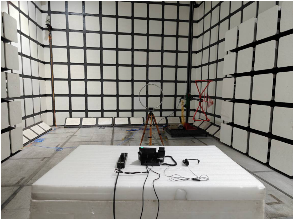
Radiated Emissions View (Below 1 GHz)_Adapter
