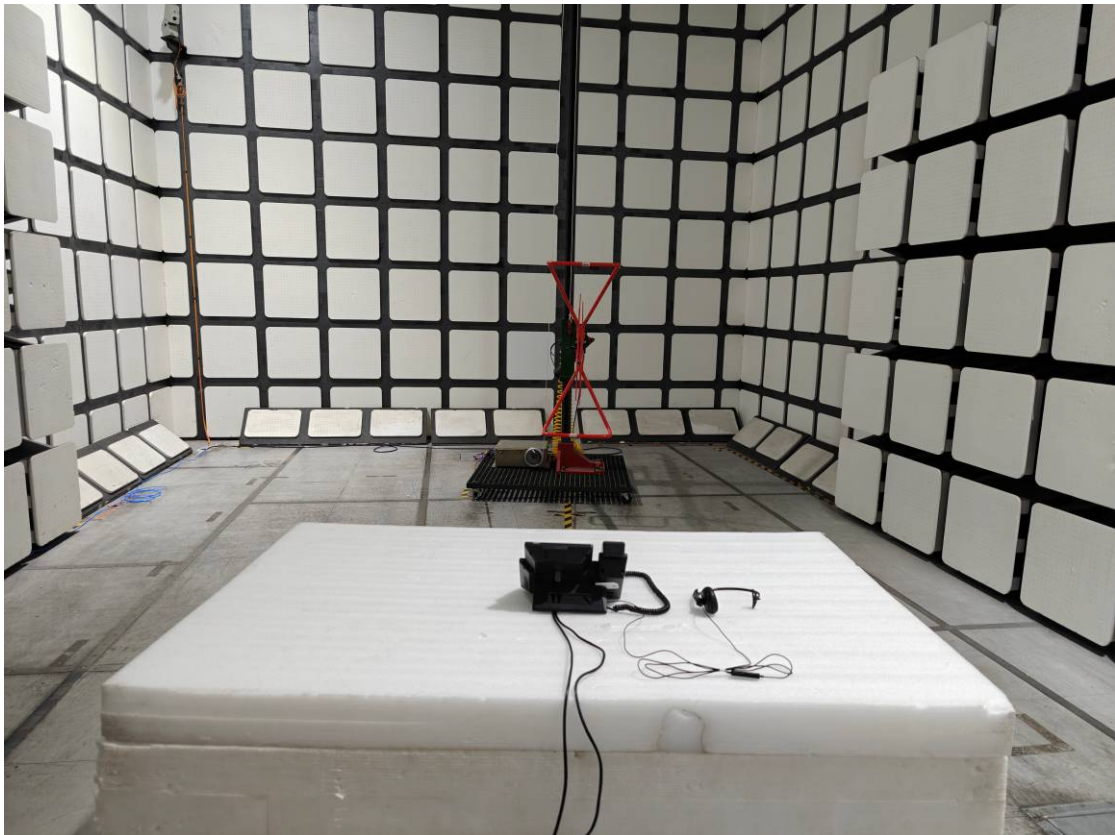
Radiated Emissions View (Below 1 GHz)_POE
