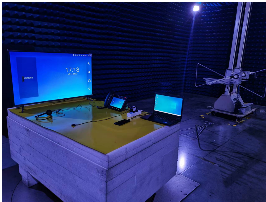
Photo of Radiated Emission Measurement (Below 1G) Powered by Adapter
