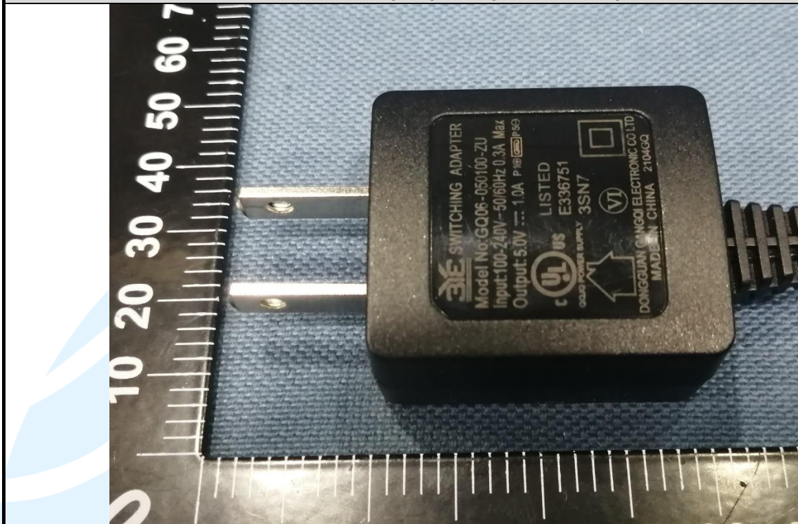
EUT Photo (Adapter GQ06-050100-ZU)
