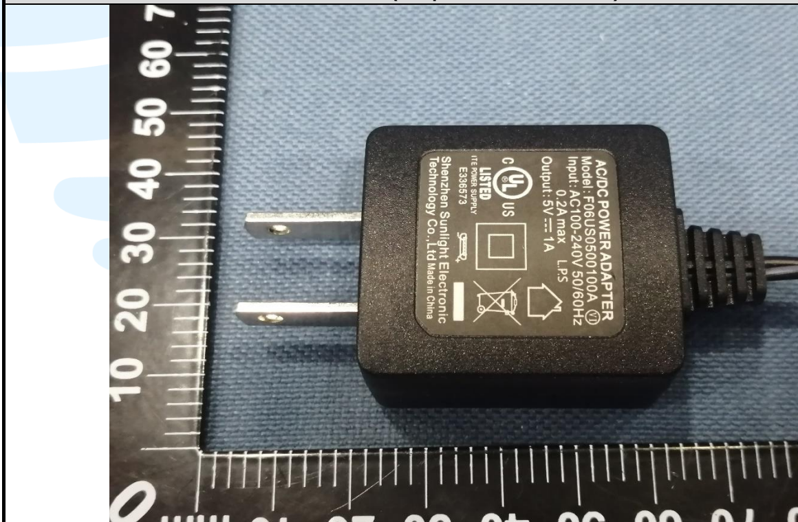
EUT Photo (Adapter F06US0500100A)
