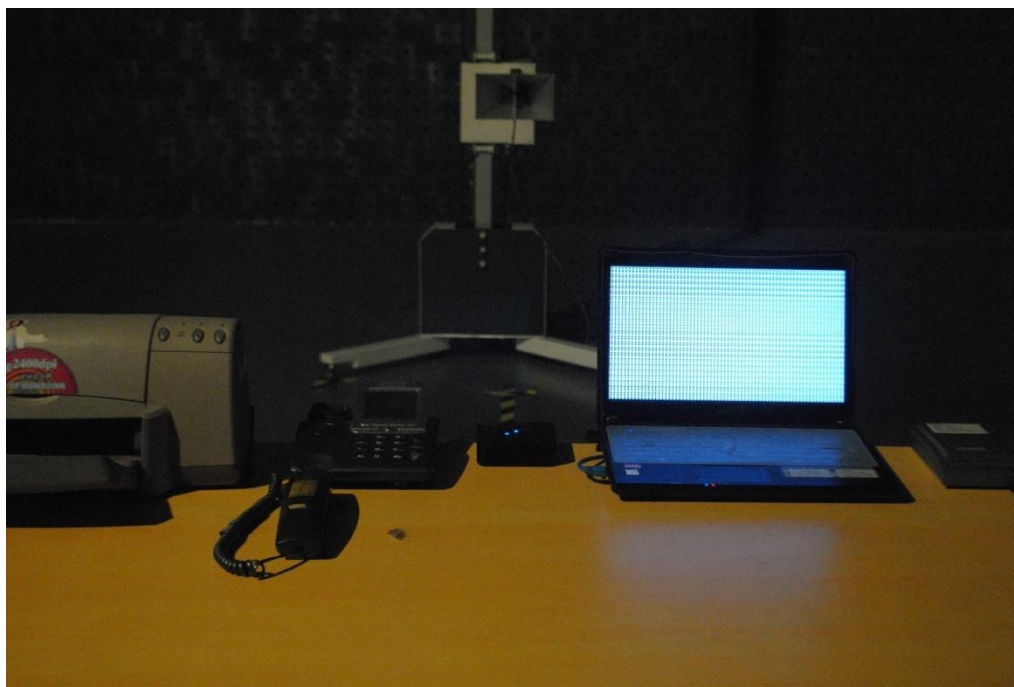
Radiated Emission test view (Above 1GHz)
