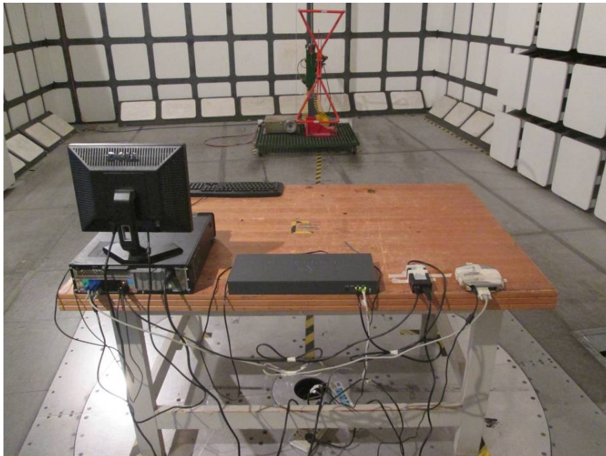
Radiated Emissions Rear View (Below 1 GHz, Power by POE)
