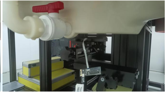
Rear Face of EUT with 1.0 cm Gap
