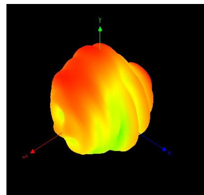
5G 3D
