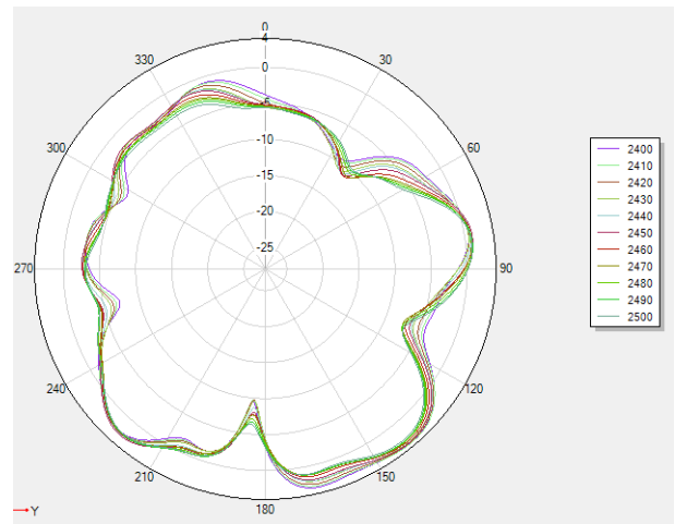
2.4G phi=90deg
