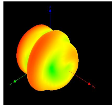
2.4G 3D
