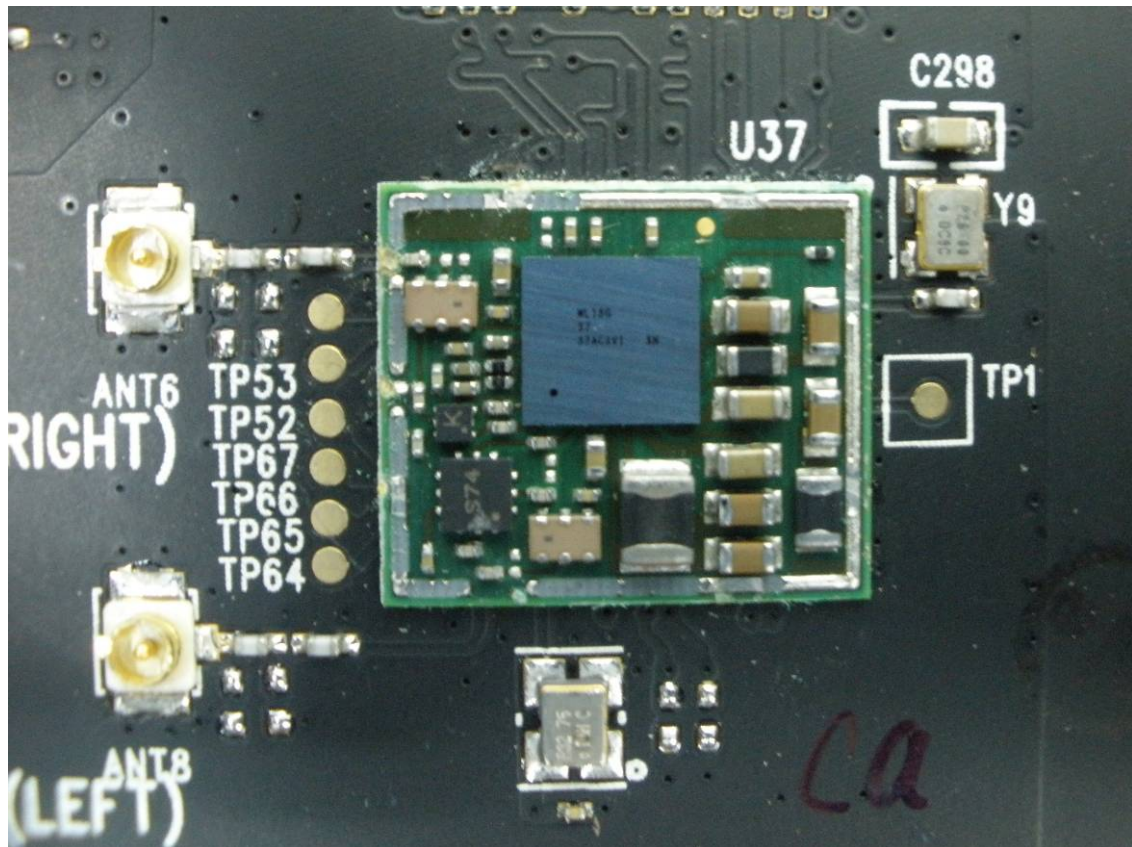
Antenna 2(chain 1)
