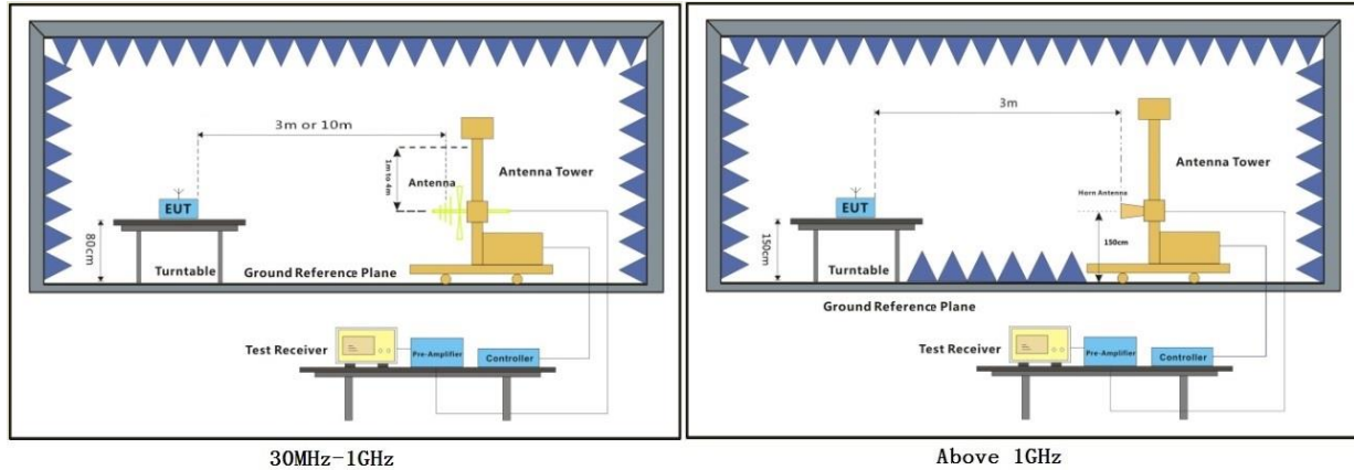
30MHz-1GHz
