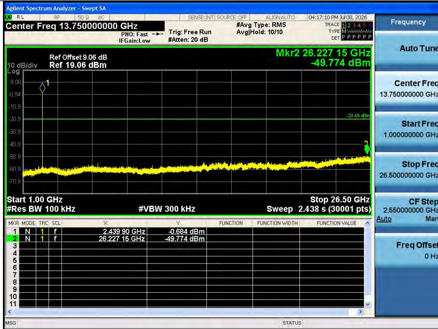
BLE_2M_Ant1_2440_1000~26500
