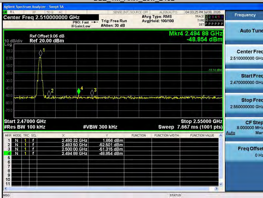
BLE_1M_Ant1_High_2480
