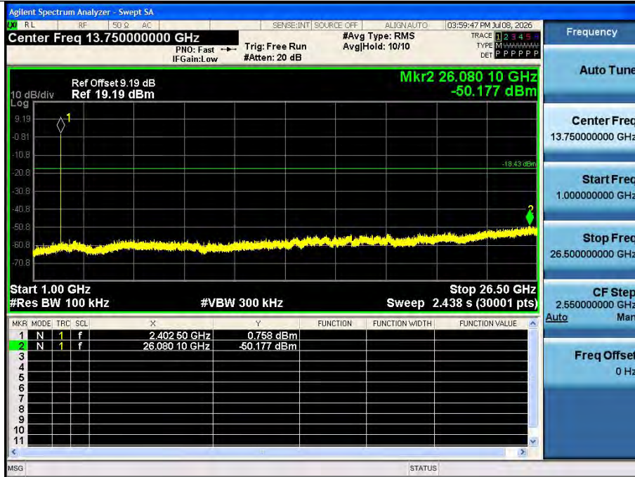
BLE_1M_Ant1_2402_1000~26500
