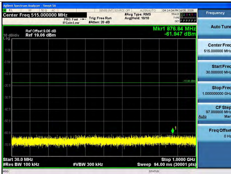
BLE_2M_Ant1_2478_30~1000
