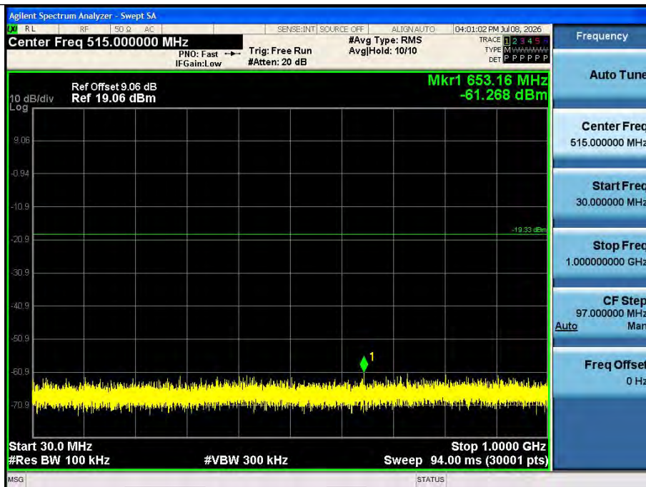
BLE_1M_Ant1_2440_30~1000
