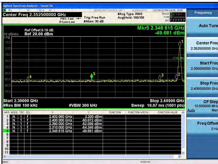
BLE_1M_Ant1_Low_2402
