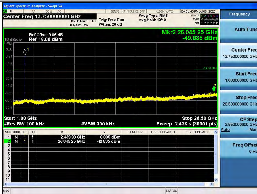
BLE_1M_Ant1_2440_1000~26500
