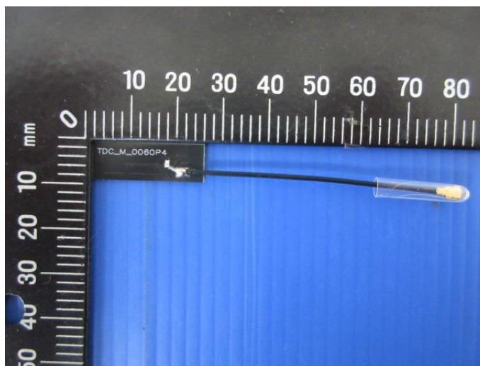
Black Antenna / (T-543-9291152-11)
