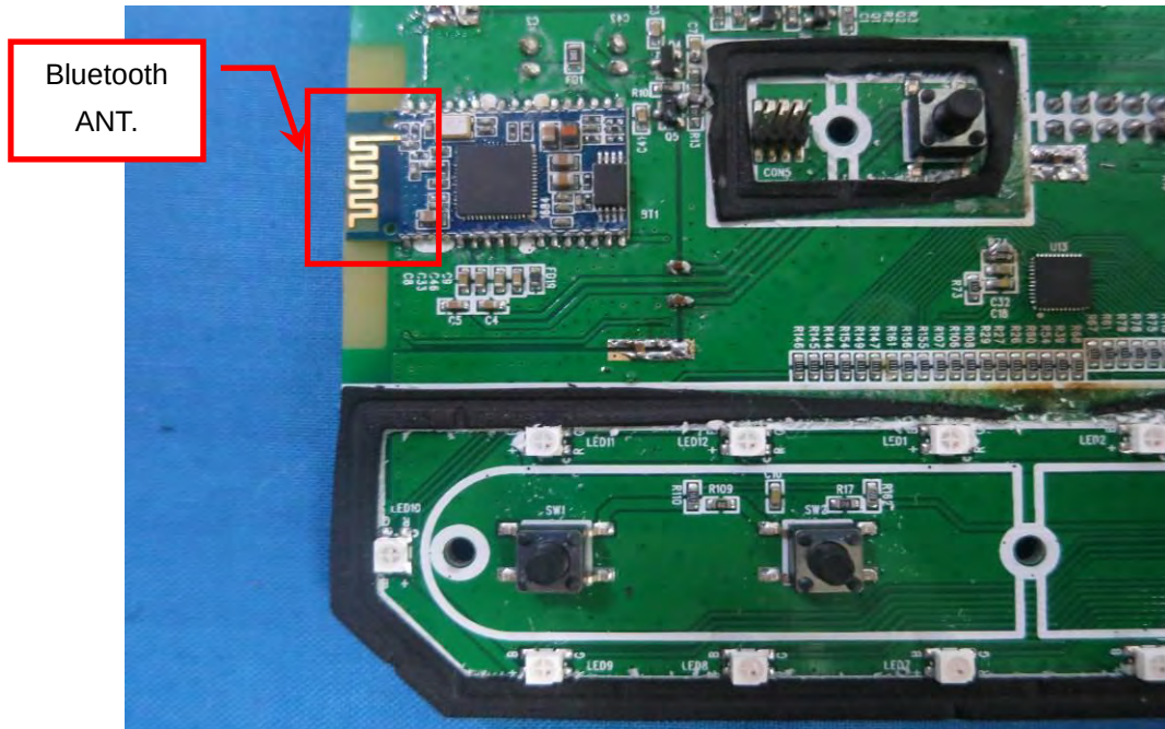
EUT Photo (26)
