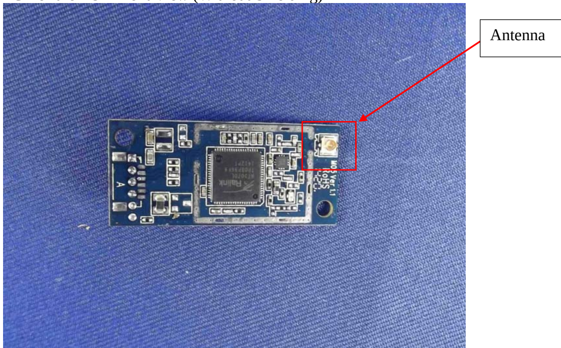
Figure 22 PCB of the EUT-Front View (Without Shielding)
