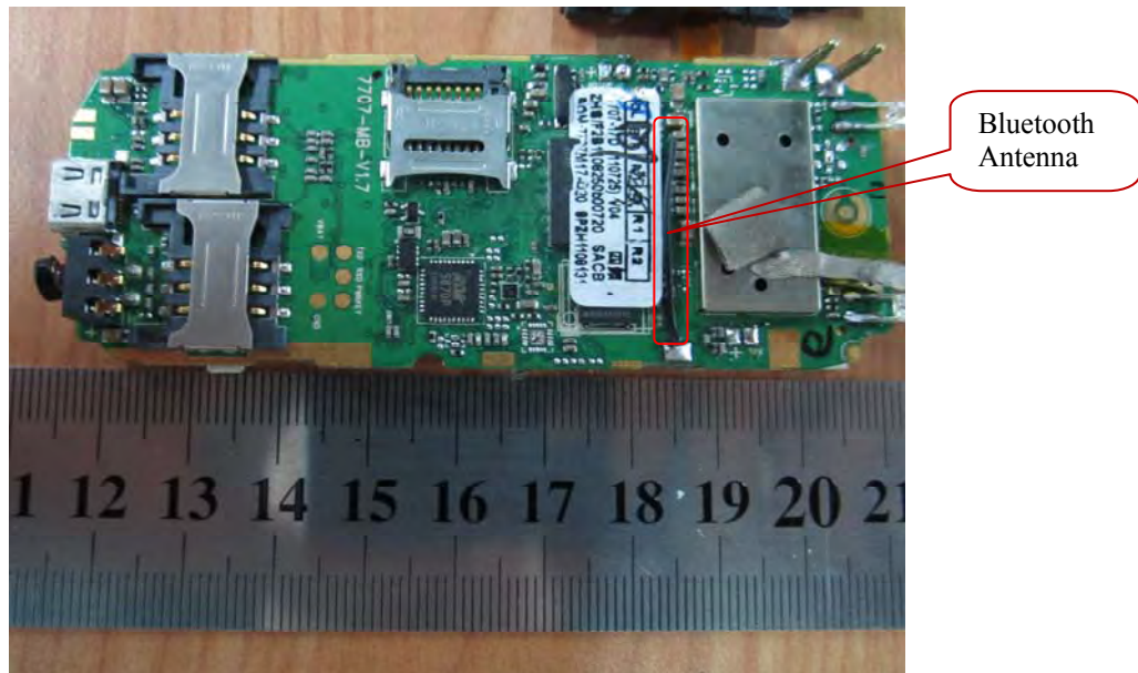
PCB Board view1
