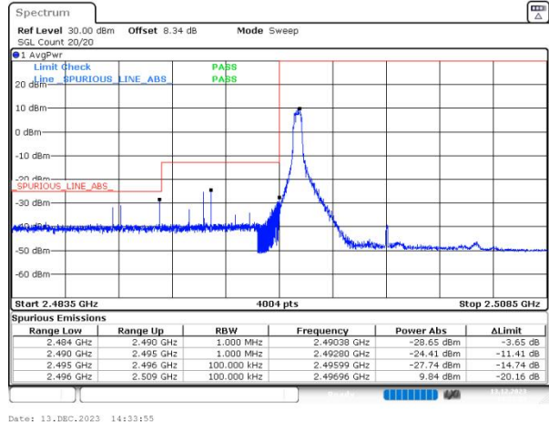
n41 SCS=30kHz DFT_256QAM BW=10MHz LowChannel=500202 RB=1@0
