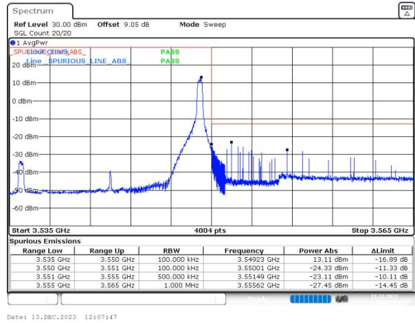
n77(3450-3550) SCS=30kHz DFT_BPSK BW=15MHz HighChannel=636166 RB=1@37
