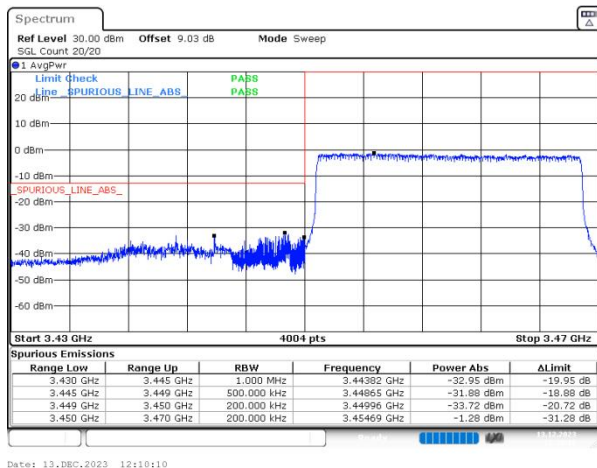
n77(3450-3550) SCS=30kHz DFT_BPSK BW=20MHz LowChannel=630668 RB=50@0
