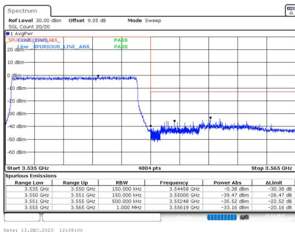
n77(3450-3550) SCS=30kHz DFT_BPSK BW=15MHz HighChannel=636166 RB=36@0
