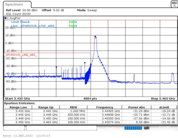
n77(3450-3550) SCS=30kHz DFT_256QAM BW=15MHz LowChannel=630500 RB=1@0
