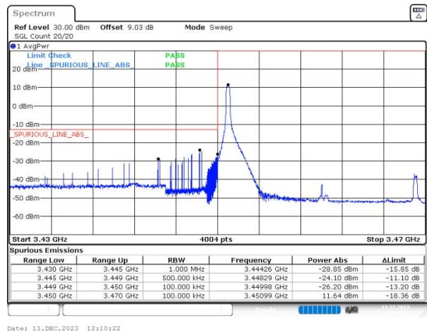
n77(3450-3550) SCS=30kHz DFT_BPSK BW=20MHz LowChannel=630668 RB=1@0
