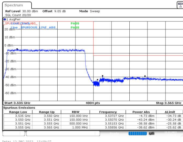
n77(3450-3550) SCS=30kHz DFT_256QAM BW=15MHz HighChannel=636166 RB=36@0
