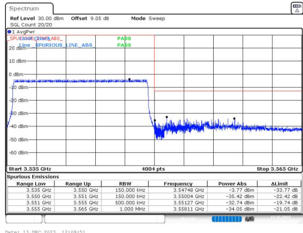
n77(3450-3550) SCS=30kHz CP_QPSK BW=15MHz HighChannel=636166 RB=38@0
