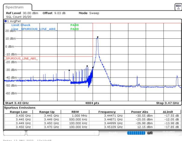
n77(3450-3550) SCS=30kHz DFT_QPSK BW=20MHz LowChannel=630668 RB=1@0
