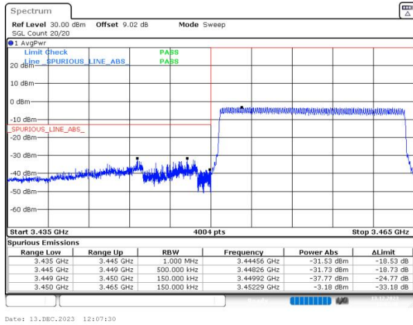
n77(3450-3550) SCS=30kHz CP_QPSK BW=15MHz LowChannel=630500 RB=38@0
