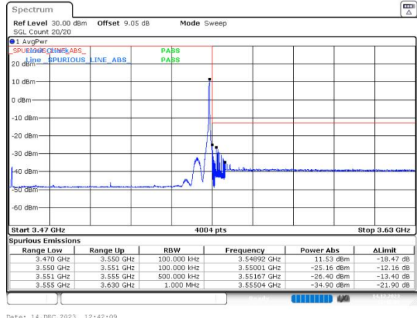
n78(3450-3550) SCS=30kHz DFT_BPSK BW=80MHz HighChannel=634000 RB=1@216
