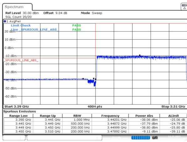
n78(3450-3550) SCS=30kHz DFT_64QAM BW=60MHz LowChannel=632000 RB=162@0
