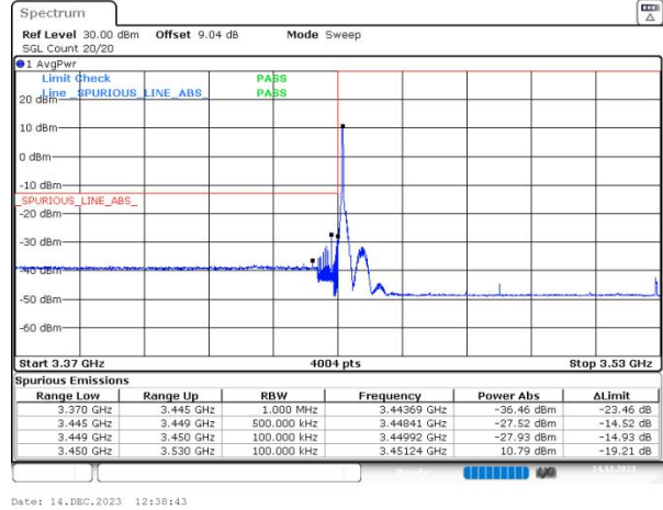
n78(3450-3550) SCS=30kHz DFT_QPSK BW=80MHz LowChannel=632668 RB=1@0
