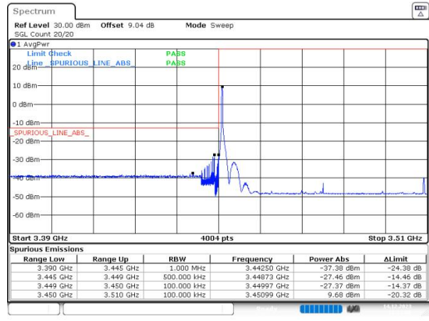
n78(3450-3550) SCS=30kHz DFT_64QAM BW=60MHz LowChannel=632000 RB=1@0
