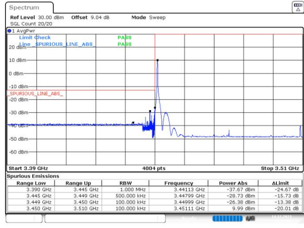
n78(3450-3550) SCS=30kHz DFT_16QAM BW=60MHz LowChannel=632000 RB=1@0
