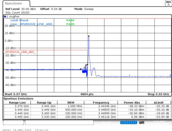
n78(3450-3550) SCS=30kHz DFT_256QAM BW=80MHz LowChannel=632668 RB=1@0
