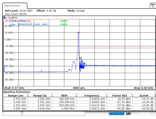
n78(3450-3550) SCS=30kHz DFT_QPSK BW=80MHz HighChannel=634000 RB=1@216
