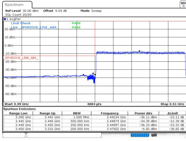
n78(3450-3550) SCS=30kHz DFT_16QAM BW=60MHz LowChannel=632000 RB=162@0
