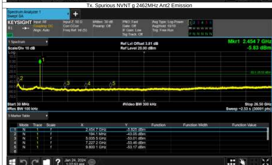
Tx. Spurious NVNT g 2462MHz Ant2 Emission
