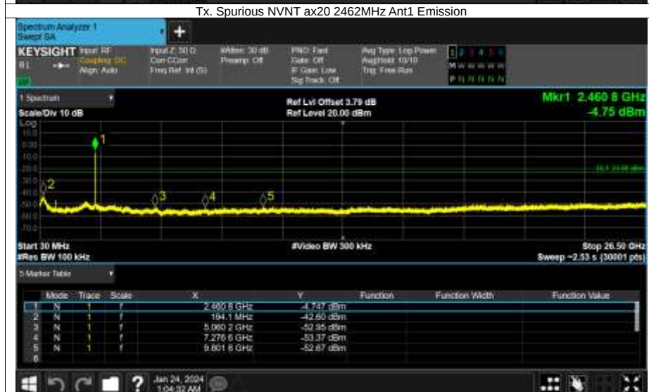
Tx. Spurious NVNT ax20 2462MHz Ant1 Emission
