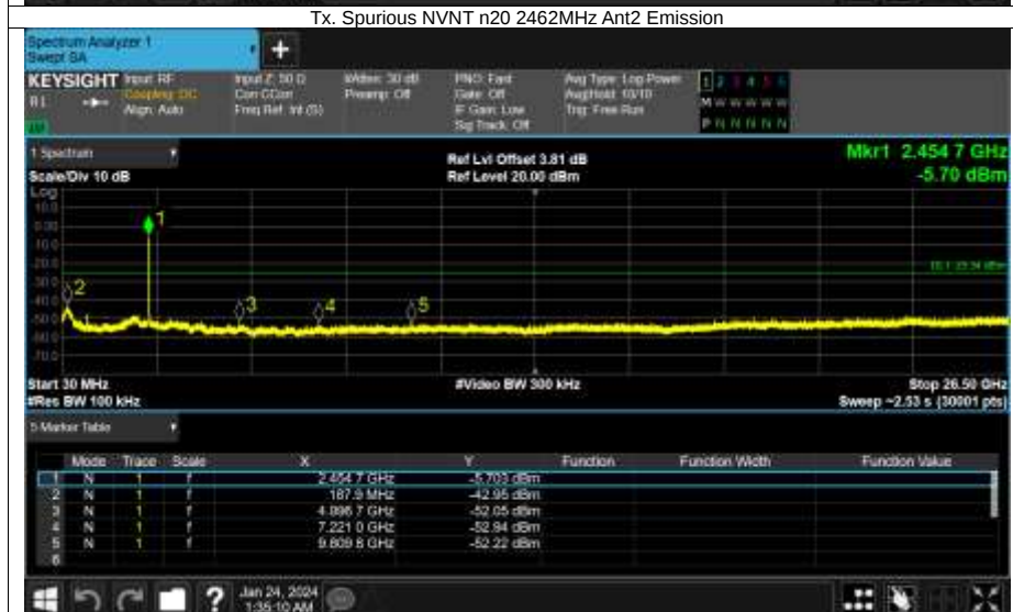
Tx. Spurious NVNT n20 2462MHz Ant2 Emission
