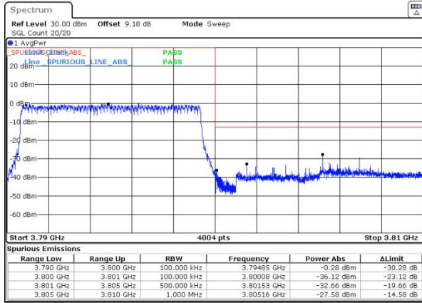
n78(3700-3800) SCS=30kHz DFT_BPSK BW=10MHz HighChannel=653000 RB=24@0
