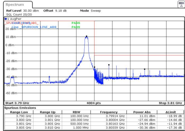
n78(3700-3800) SCS=30kHz DFT_QPSK BW=10MHz HighChannel=653000 RB=1@23
