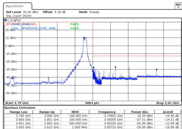
n78(3700-3800) SCS=30kHz DFT_16QAM BW=10MHz HighChannel=653000 RB=1@23
