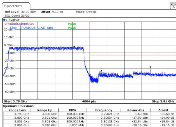
n78(3700-3800) SCS=30kHz DFT_QPSK BW=10MHz HighChannel=653000 RB=24@0
