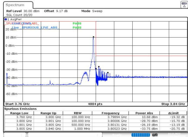
n78(3700-3800) SCS=30kHz DFT_QPSK BW=40MHz HighChannel=652000 RB=1@105
