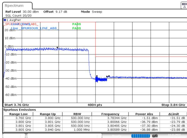
n78(3700-3800) SCS=30kHz DFT_QPSK BW=40MHz HighChannel=652000 RB=100@0
