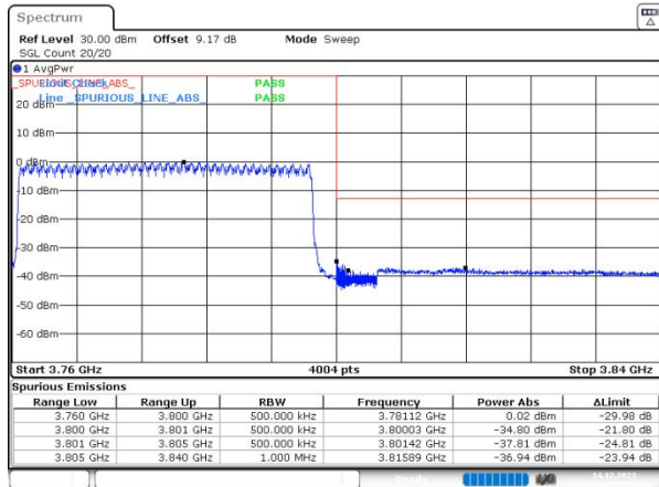
n78(3700-3800) SCS=30kHz DFT_BPSK BW=40MHz HighChannel=652000 RB=100@0
