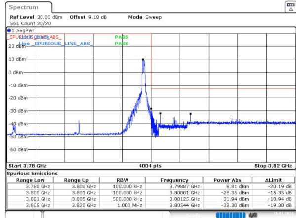
n78(3700-3800) SCS=30kHz DFT_64QAM BW=20MHz HighChannel=652666 RB=1@50
