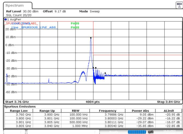
n78(3700-3800) SCS=30kHz DFT_16QAM BW=40MHz HighChannel=652000 RB=1@105
