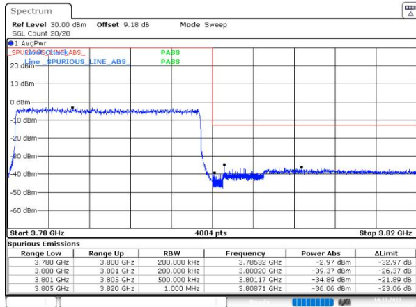
n78(3700-3800) SCS=30kHz DFT_16QAM BW=20MHz HighChannel=652666 RB=50@0
