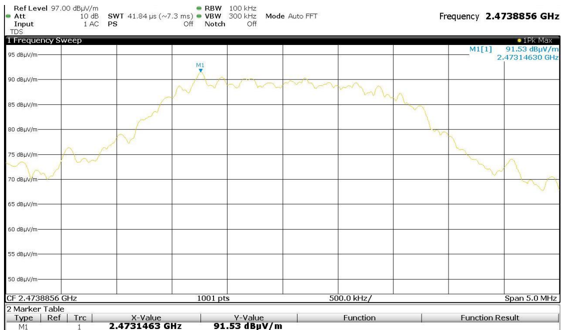
Channel 2474 MHz
