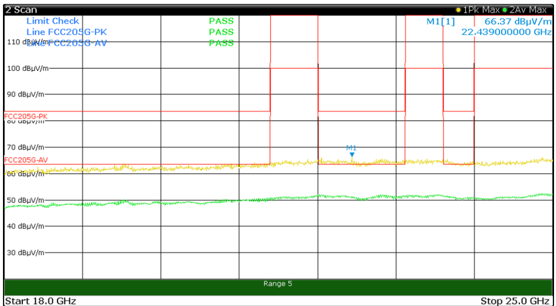
Channel 2438 MHz
