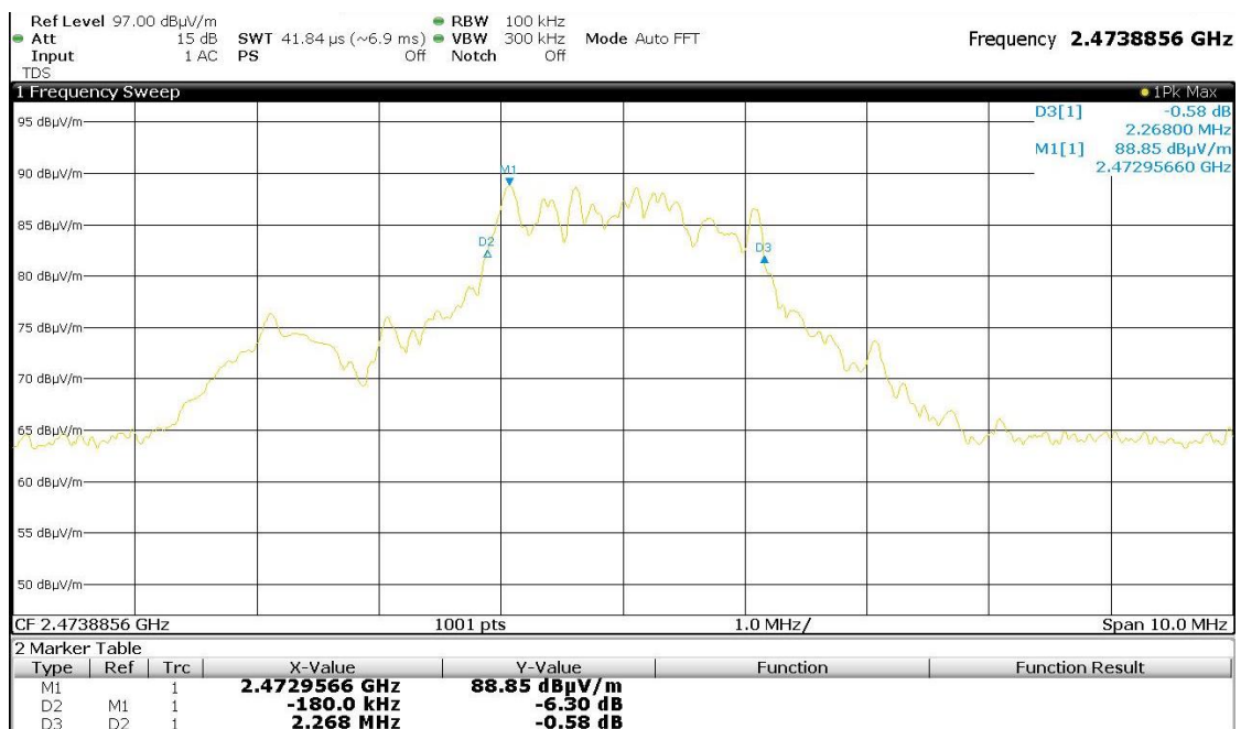
Channel 2474 MHz
