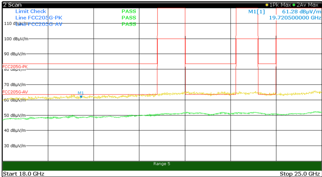
Channel 2406 MHz
