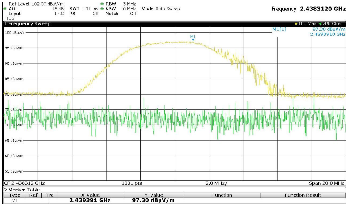
Channel 2438 MHz
