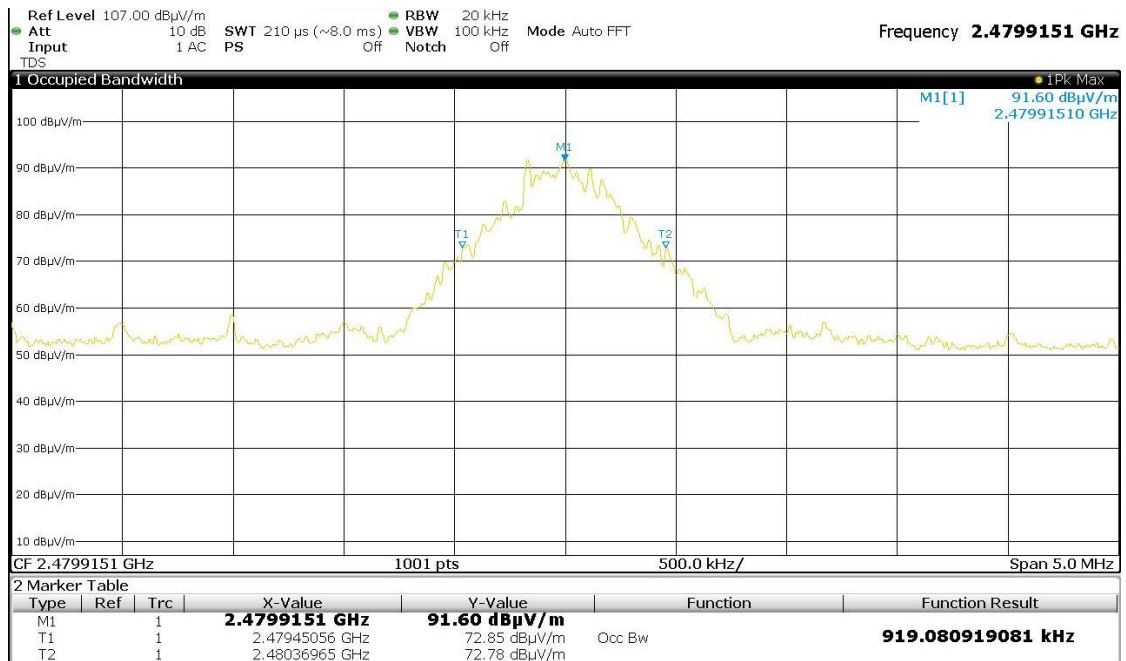
Channel 2480 MHz
