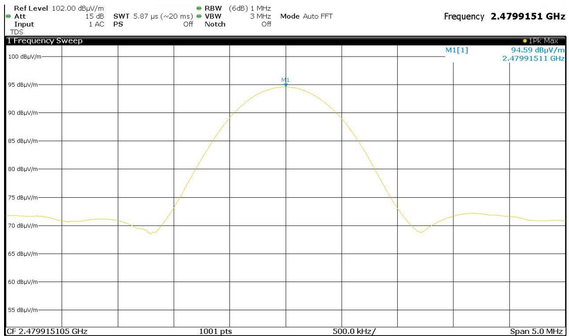
Channel 2480 MHz
