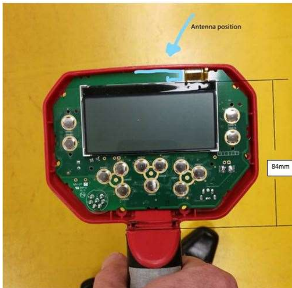
Distance of Internal Antenna to Handle
