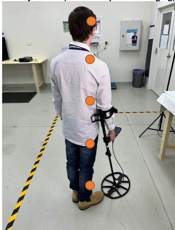
Survey Point 8 (E/H-Field Spatial Averaging)
