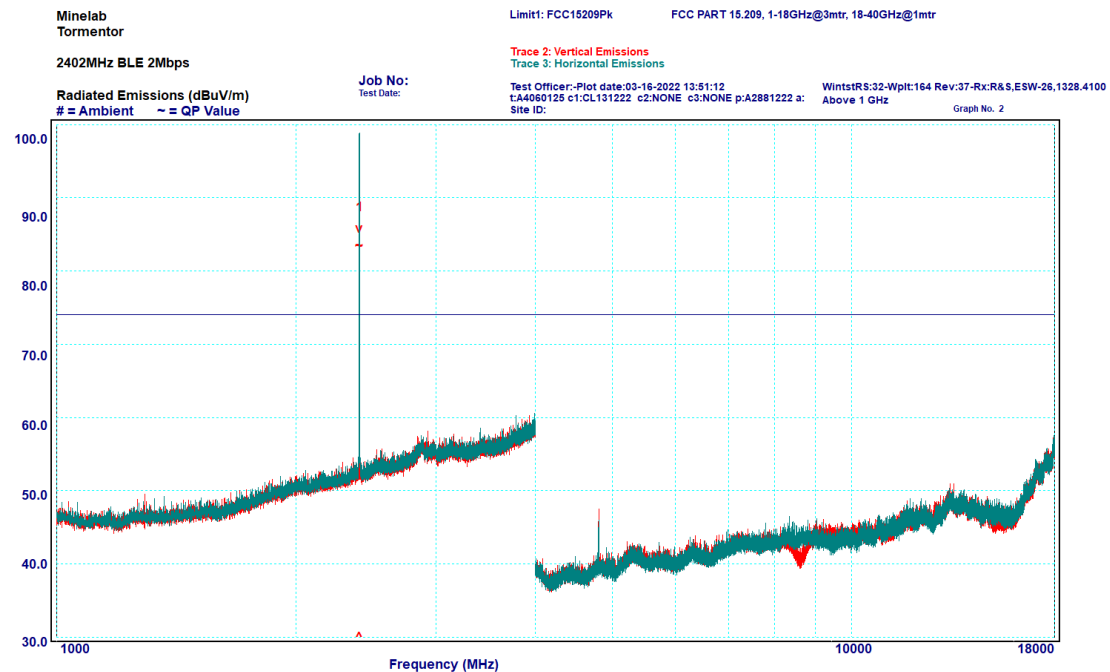
Graph 6-6: Transmitter Spurious Emissions, 1 – 18 GHz, 2402 MHz, Peak
