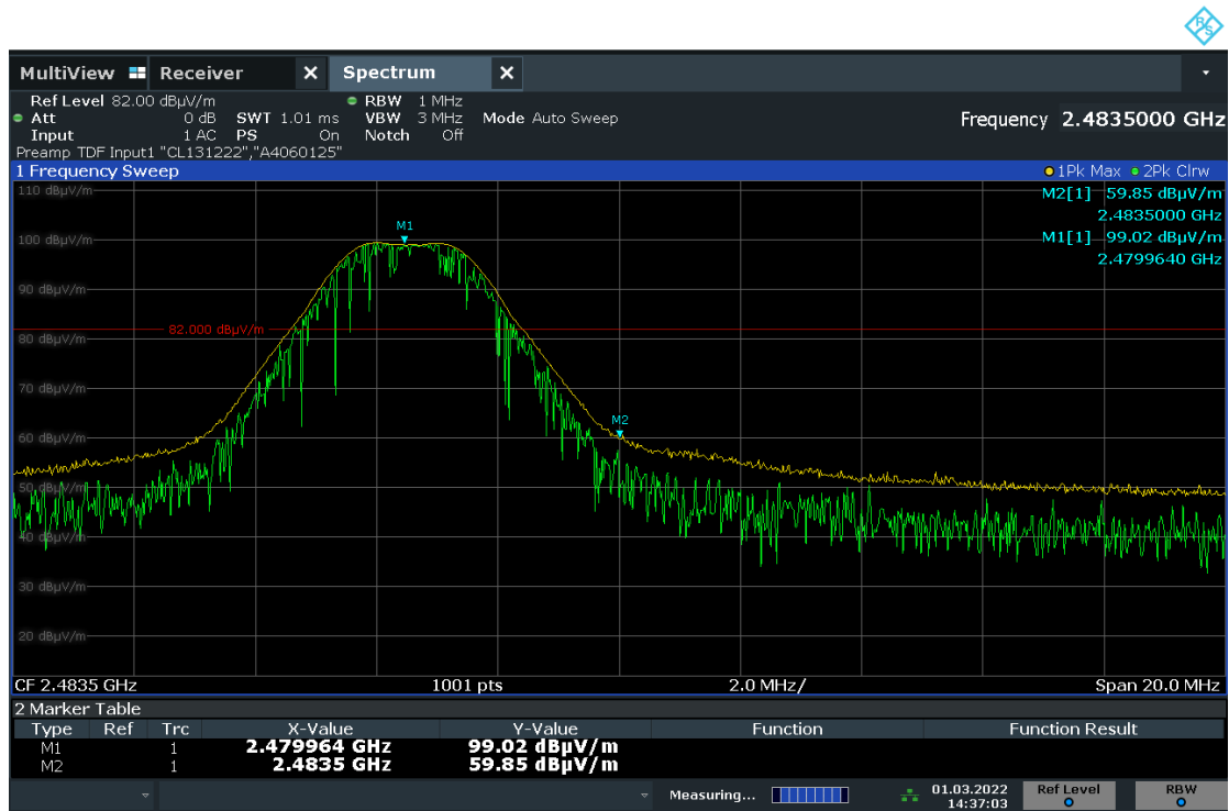
Graph 6-11: Band Edge Emission, Upper Band-edge, Peak
