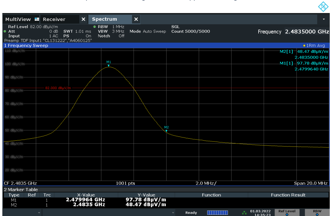
Graph 6-11: Band Edge Emission, Upper Band-edge, Peak
