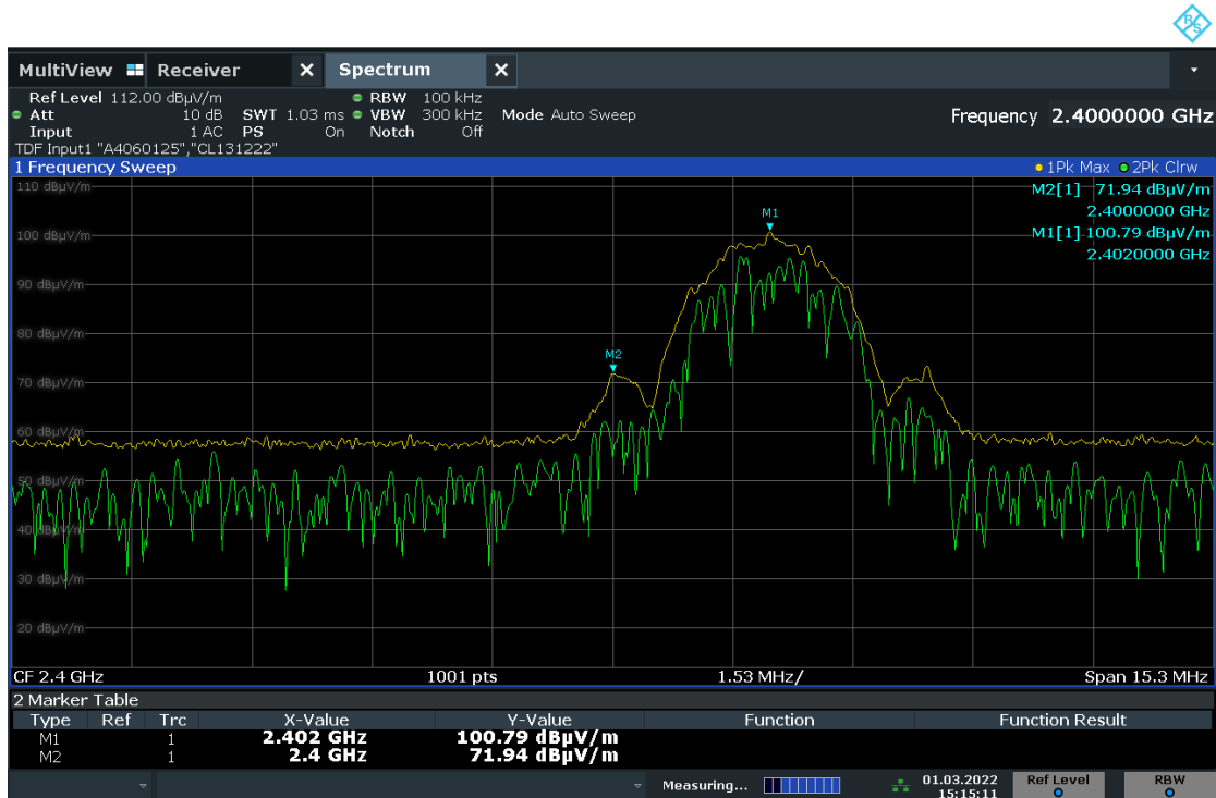
Graph 6-10: Band Edge Emission, Lower Band-edge
