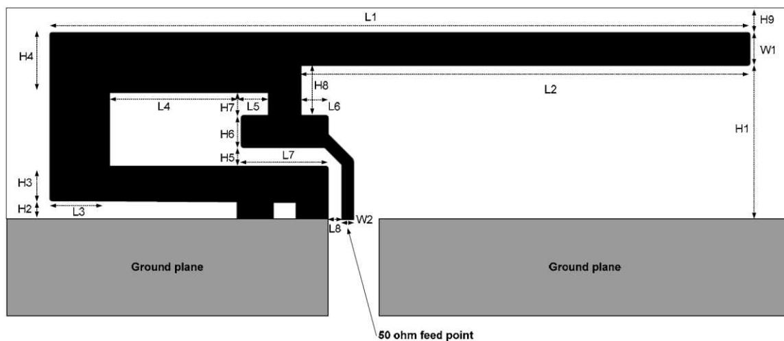
Figure 1. IFA Dimensions
