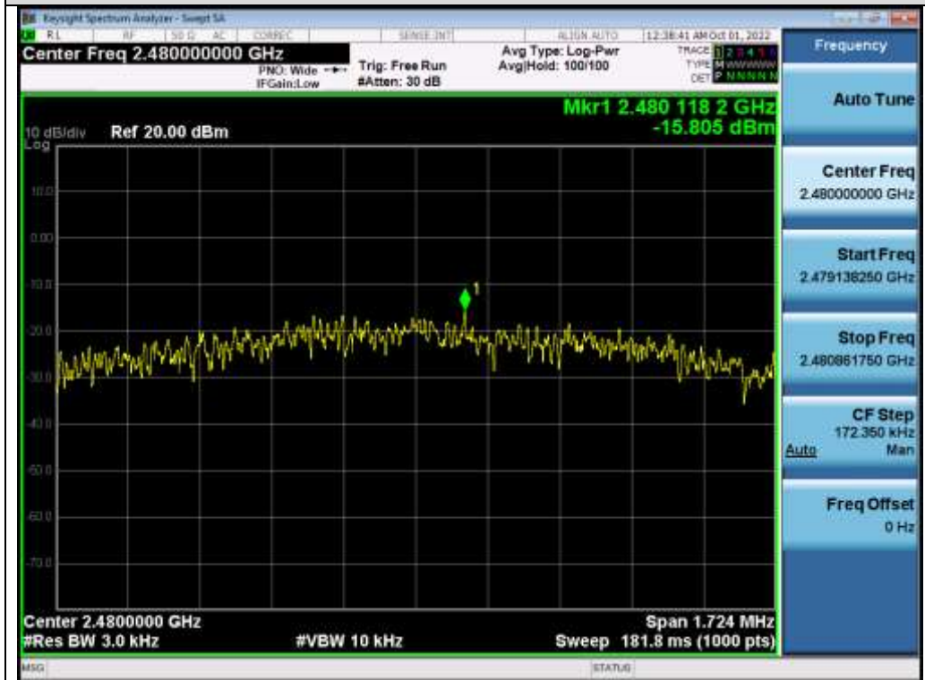
Test_Graph_LE2M_ANT1_2480_2Mbps_PSD
