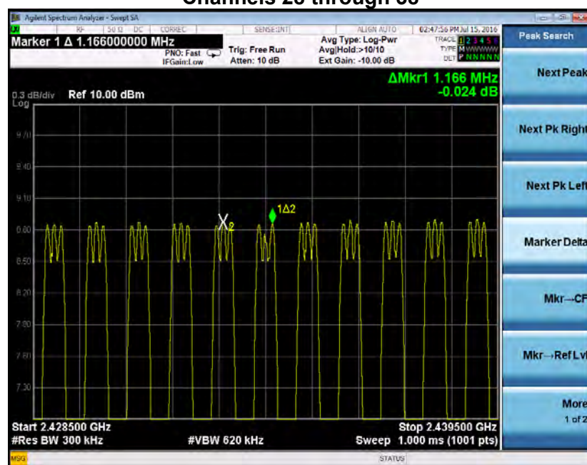
Channels 28 through 38
