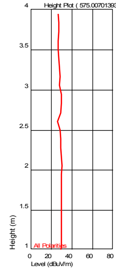
Height Plot ( 575.00701393 MHz )
