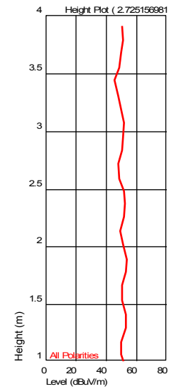
Height Plot ( 2.725156981 GHz )
