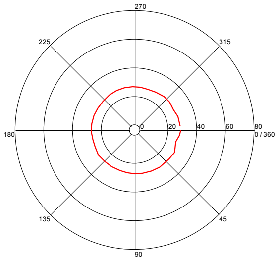
Turntable Plot ( 474.974749898 MHz )
