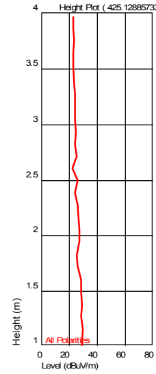
Height Plot ( 425.128857335 MHz )
