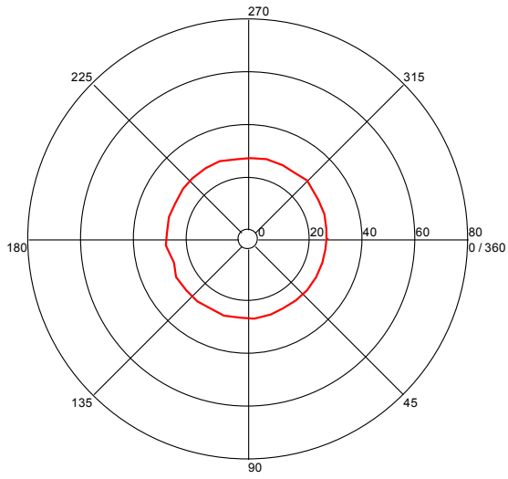
Turntable Plot ( 125.001803549 MHz )
