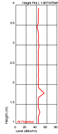
Height Plot ( 1.907107548 GHz )
