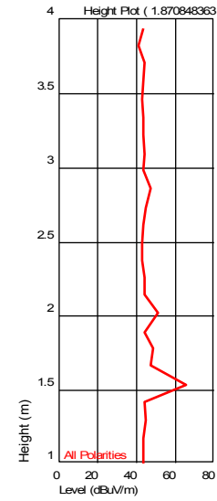
Height Plot ( 1.870848363 GHz )
