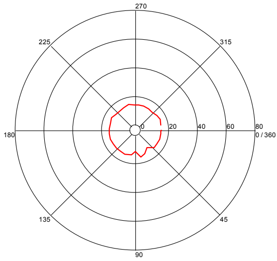
Turntable Plot ( 74.227655473 MHz )
