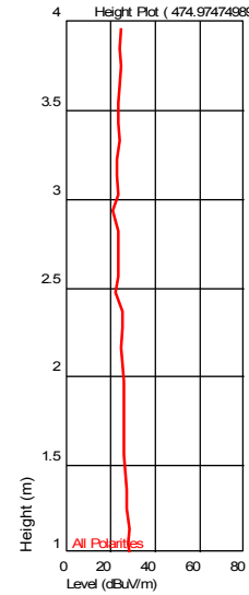
Height Plot ( 474.974749898 MHz )
