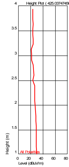
Height Plot ( 425.037474569 MHz )
