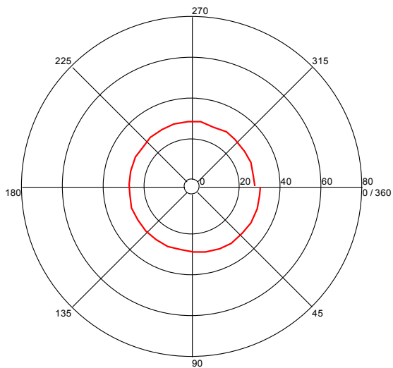
Turntable Plot ( 450.025651784 MHz )
