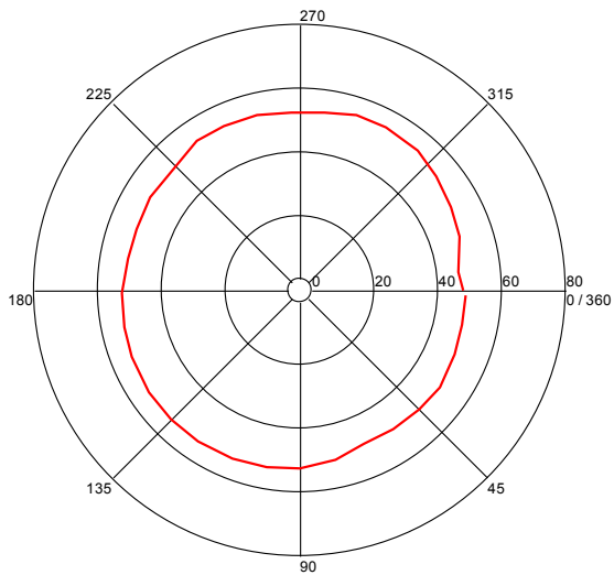
Turntable Plot ( 2.725156981 GHz )
