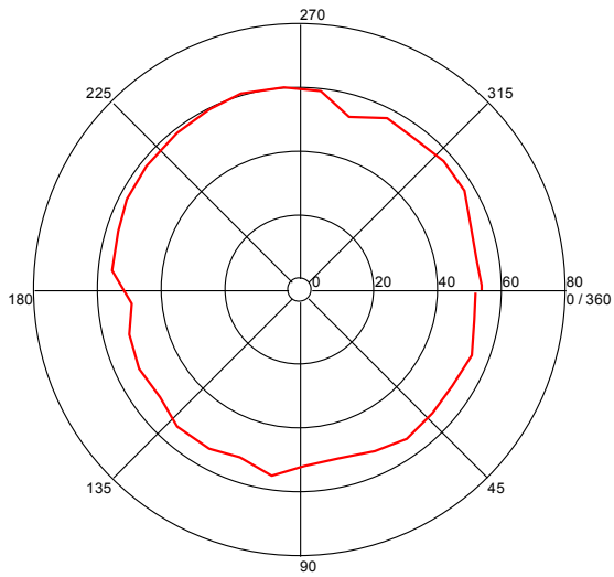
Turntable Plot ( 6.358643955 GHz )
