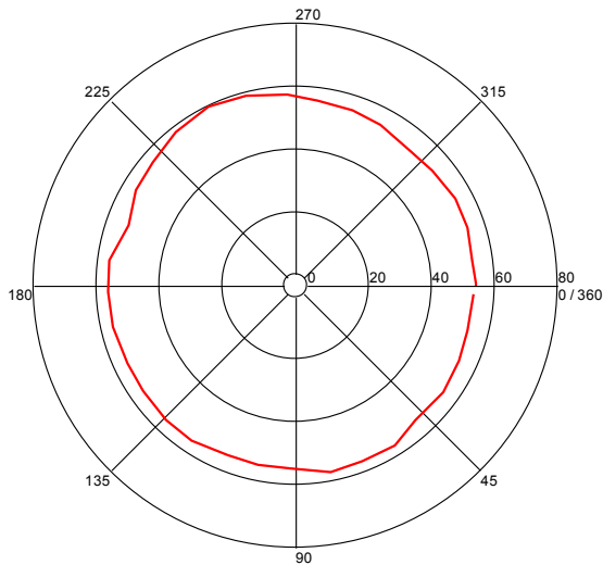
Turntable Plot ( 9.992177689 GHz )
