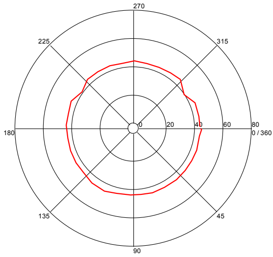
Turntable Plot ( 1.907107548 GHz )
