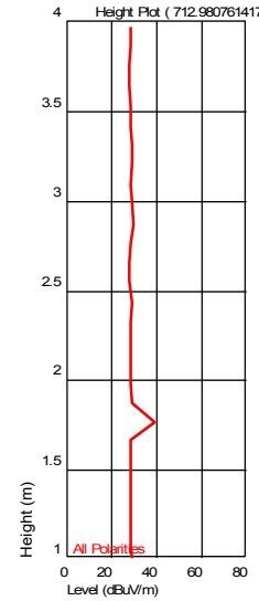
Height Plot ( 712.980761417 MHz )
