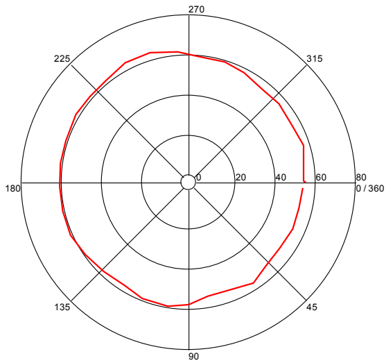
Turntable Plot ( 6.358537074 GHz )
