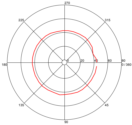
Turntable Plot ( 1.870848363 GHz )
