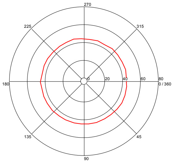
Turntable Plot ( 2.436392785 GHz )
