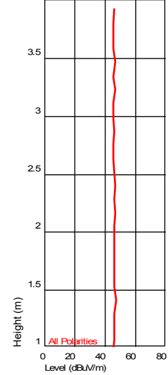
Height Plot ( 2.947688711 GHz )
