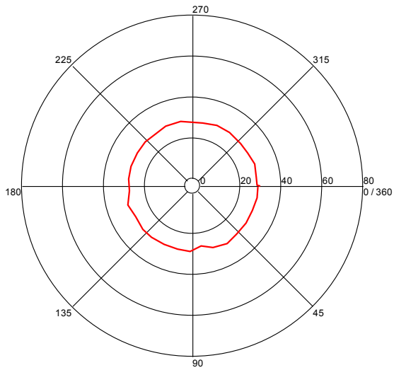
Turntable Plot ( 712.980761417 MHz )
