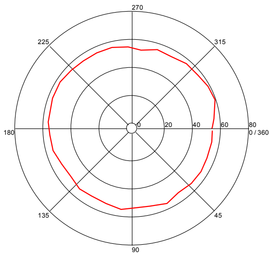
Turntable Plot ( 9.992625251 GHz )
