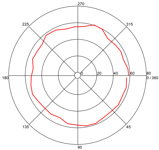
Turntable Plot ( 6.358603875 GHz )
