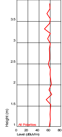
Height Plot ( 6.358603875 GHz )
