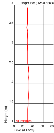
Height Plot ( 125.001803549 MHz )
