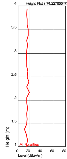
Height Plot ( 74.227655473 MHz )
