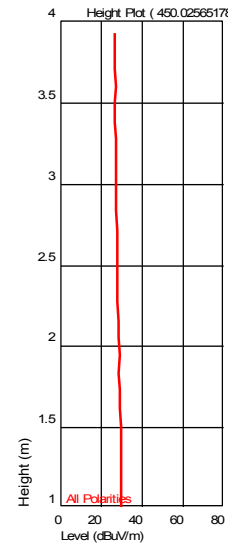
Height Plot ( 450.025651784 MHz )
