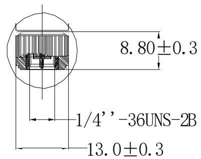
SMA-Male DETAIL A SCALE 2:1
