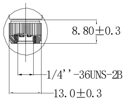
SMA-Female DETAIL A SCALE 2:1
