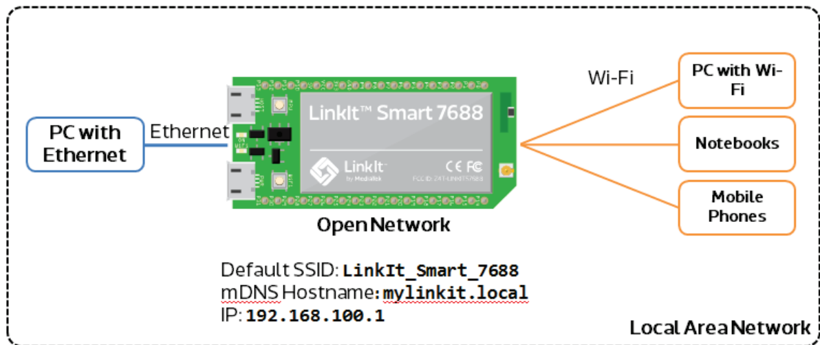
Figure 9 LinkIt Smart 7688 in AP Mode
