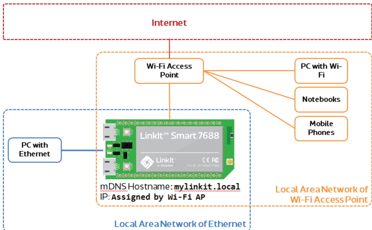
Figure 10 LinkIt Smart 7688 in Station Mode
