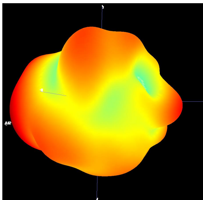
B1.2 3D Pattern for 910MHz
