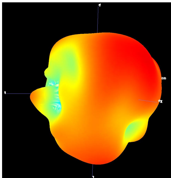
B1.1 3D Pattern for 890MHz
