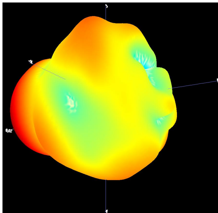
B1.3 3D Pattern for 930MHz
